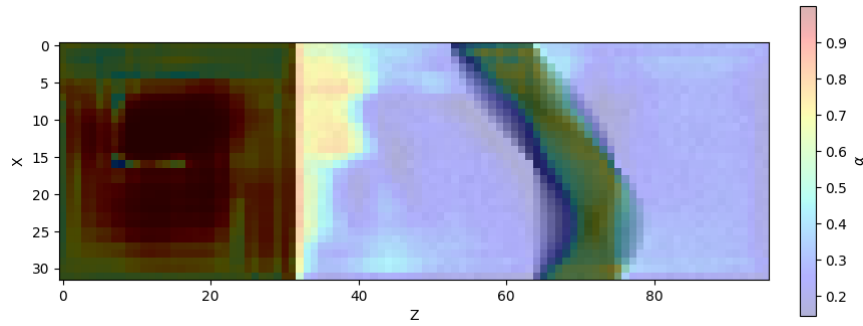
Figure 16: An attention map illustrating the regions of the input data that the attention mechanism in the first skip connection of the AttU-Net focuses on. The image was generated by running the model on a phantom and extracting the values of the attention coefficients \alpha . A 2D slice (at y = 16 ) was taken from the 3D attention volume.
