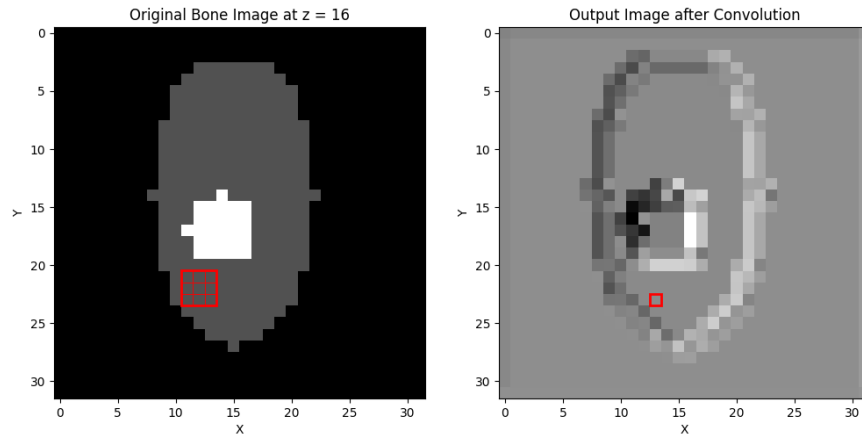
Figure 7: left : original phantom with a 2D 3x3 randomly initialised kernel drawn on top. each individual square represents a pixel, with the outer square representing the kernel. right : phantom after 2D convolution layer has been applied.
