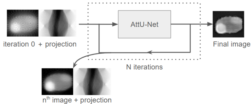
Figure 11: Schematic overview of the model workflow. The input to the model consists of the initial reconstructed image from iteration 0 combined with the corresponding projection (sinogram) data. The network processes this input iteratively, where the output of the n^{th} iteration is used as the input for the (n + 1)^{th} iteration, while the projection data remains constant. After N iterations, the final reconstructed image is produced.
