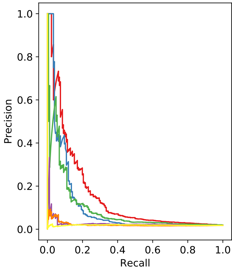
Precision-Recall — DREAM4
