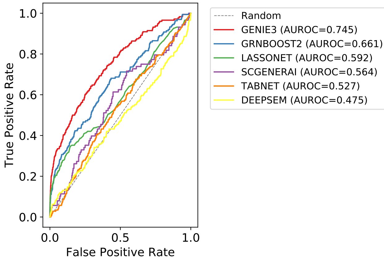
ROC Curve — DREAM4
