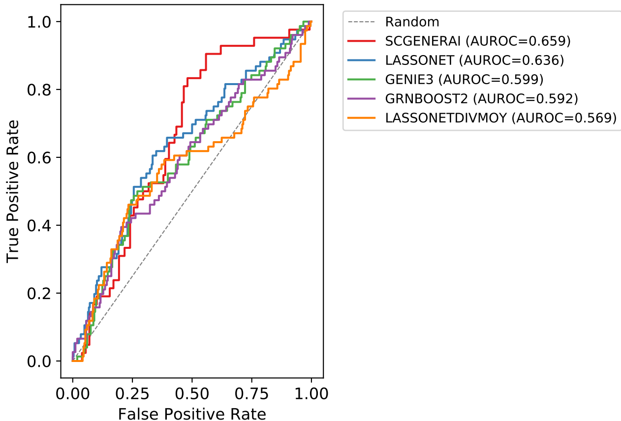
ROC Curve — GSD
