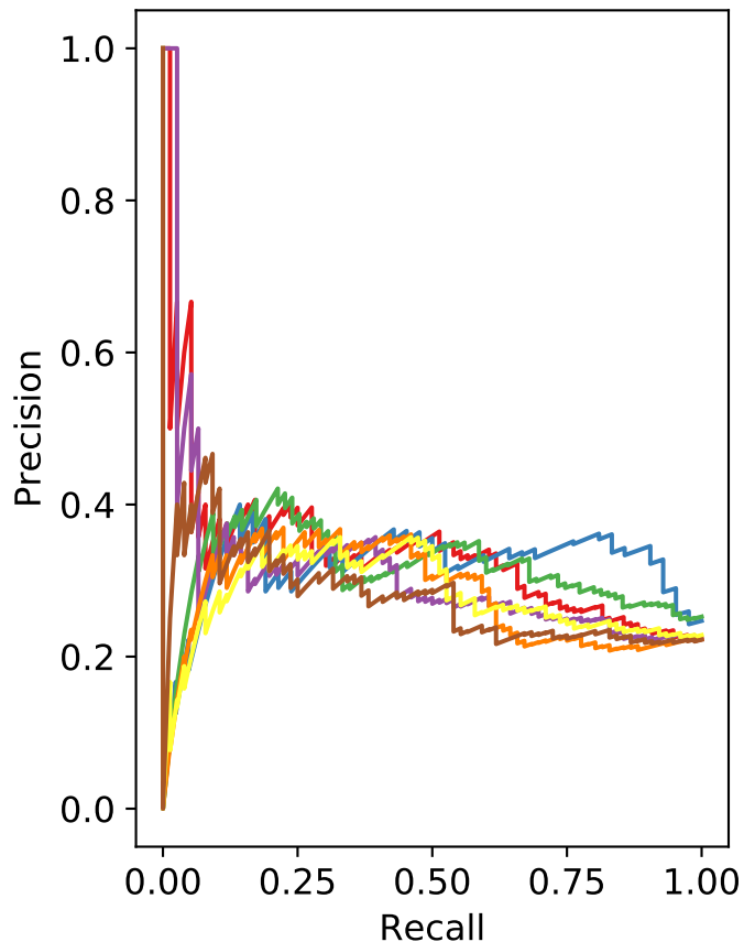
Precision-Recall — GSD
