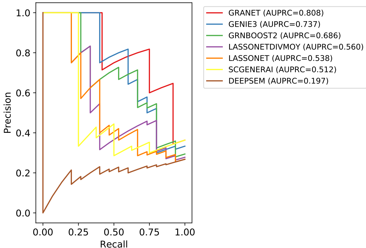
Precision-Recall — VSC
