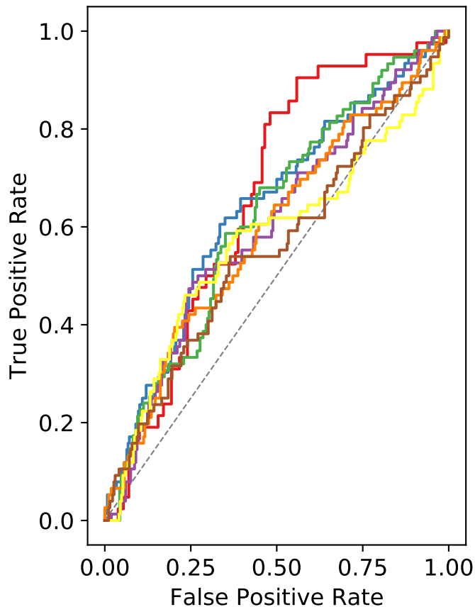
ROC Curve — GSD
