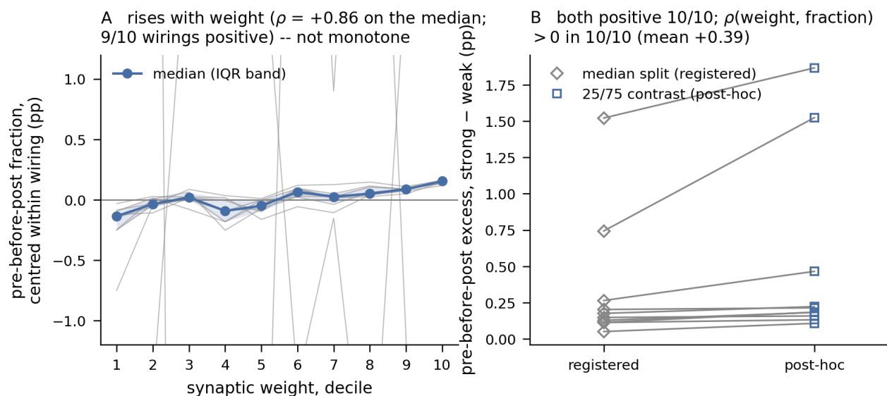
Figure S1 — Weight as a continuous predictor [exploratory, post-hoc — not registered]. (figS1_continuous_weight.pdf, from the persisted out-of-sample runs via experiments/dish/pm4_posthoc.py.) A , pre-before-post pair fraction, centred within each wiring,
