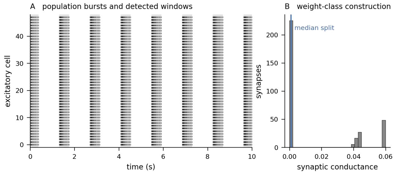
Figure 1 — The preparation and its instruments. (fig1_preparation.pdf, from stg_pm_s*.json.) A , raster of the 48 excitatory cells over 10 s of a 60 s run, with the detected burst windows shaded; bursts are delimited at full width at 20% of each burst's own peak. B , the distribution of plastic recurrent conductances at the end of the same run, with the median split that defines the strong and weak classes. A wiring in the modal bursting regime is shown; the two off-regime wirings identified in Section 2.2 differ in burst count and in the fraction of weights driven to zero, and would not be representative.
