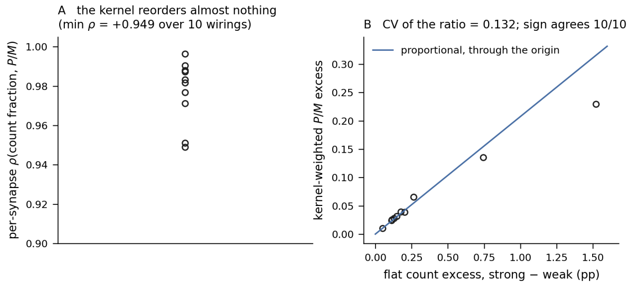
Figure S2 — Kernel ablation: flat count versus exponential kernel [exploratory, post-hoc — not registered]. (figS2_kernel_ablation.pdf, same source.) A , per-synapse rank correlation between the flat pre-before-post count fraction and the kernel-weighted P/M, one point per wiring (mean +0.977). B , kernel-weighted P/M excess against flat pre-before-post count excess (strong – weak), one point per wiring, with the proportional line through the origin at the mean per-wiring ratio; the across-wiring CV of that ratio is 0.132 (Section 2.3 reports 0.13), and the sign agrees in 10 of 10.
