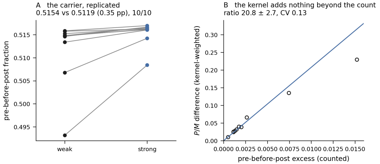
Figure 3 — The associated statistic, replicated out of sample. (fig3_carrier.pdf, from stg_pm4_s*.json.) A , pre-before-post pair fraction by class in each of the ten fresh wirings: 0.5154 against 0.5119, a 0.35-percentage-point excess on strong synapses, same sign in 10 of 10. Per-class values were not persisted for the original cohort, so this figure shows the replication rather than the original result; the two cohorts' excesses (0.22 percentage points in the original cohort, 0.35 in the replication) are independent estimates on different wirings. B , the kernel-weighted P/M difference against the counted pre-before-post excess, one point per wiring, with a proportional line through the origin at the mean per-wiring ratio (not a least-squares fit): the ratio is 20.8 \pm 2.7 (CV 0.13), so the exponential STDP weighting contributes little beyond the count under the present rule.
