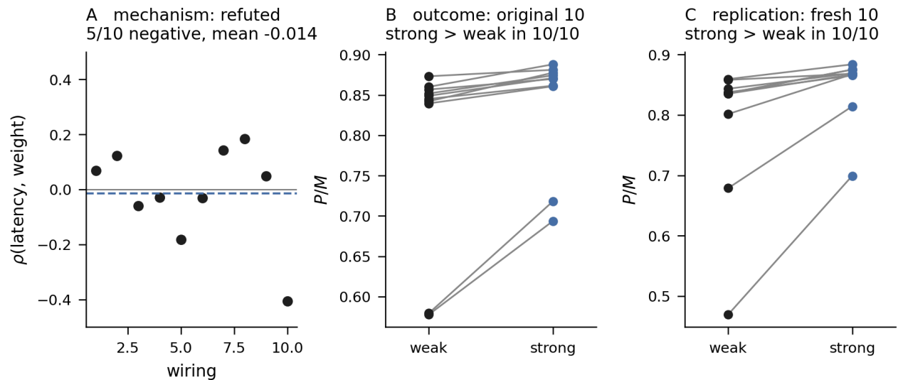
Figure 2 — The temporal mechanism is not supported; the directional outcome is. (fig2_mechanism_outcome.pdf, from stg_pm_s*.json and stg_pm4_s*.json.) A , Spearman \rho between a cell's median within-burst first-spike latency and its total incoming weight, one point per wiring, against the requirement of \geq 8/10 negative: 5 of 10 are negative and the mean (dashed) is -0.014 . B , paired weak \rightarrow strong P/M within each of the ten original wirings. C , the same on the ten
