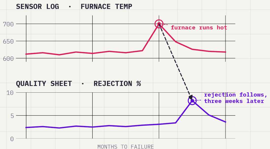
Fig. 05 / a furnace-temp spike in the sensor log predicts a rejection spike in the quality sheet, three weeks later.
