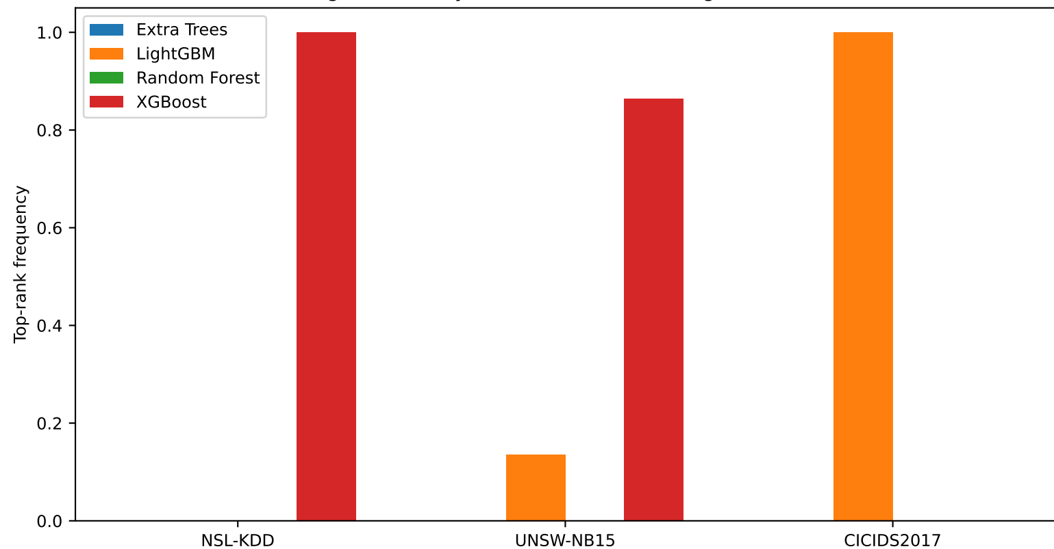
Weight sensitivity of frozen RAISE-IDS Stage-2 selection
