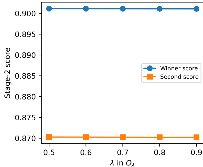
CICIDS2017
