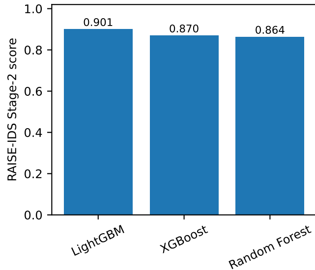
CICIDS2017
