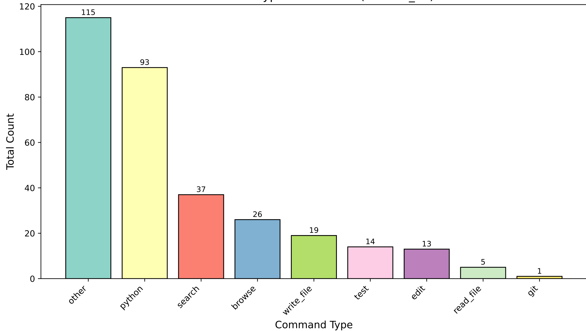
Command Type Distribution (verified_20)
