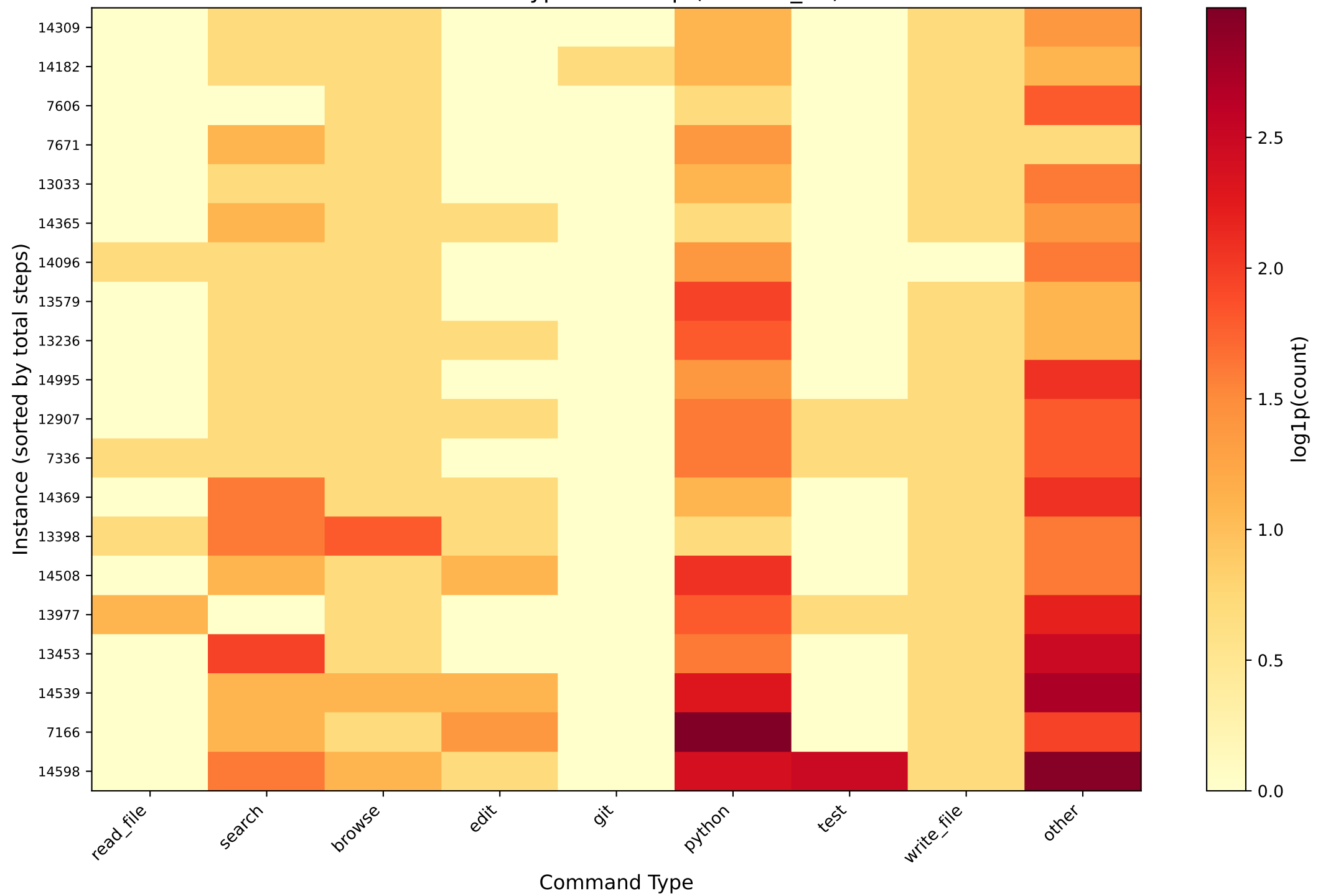
Command Type Heatmap (verified_20)
