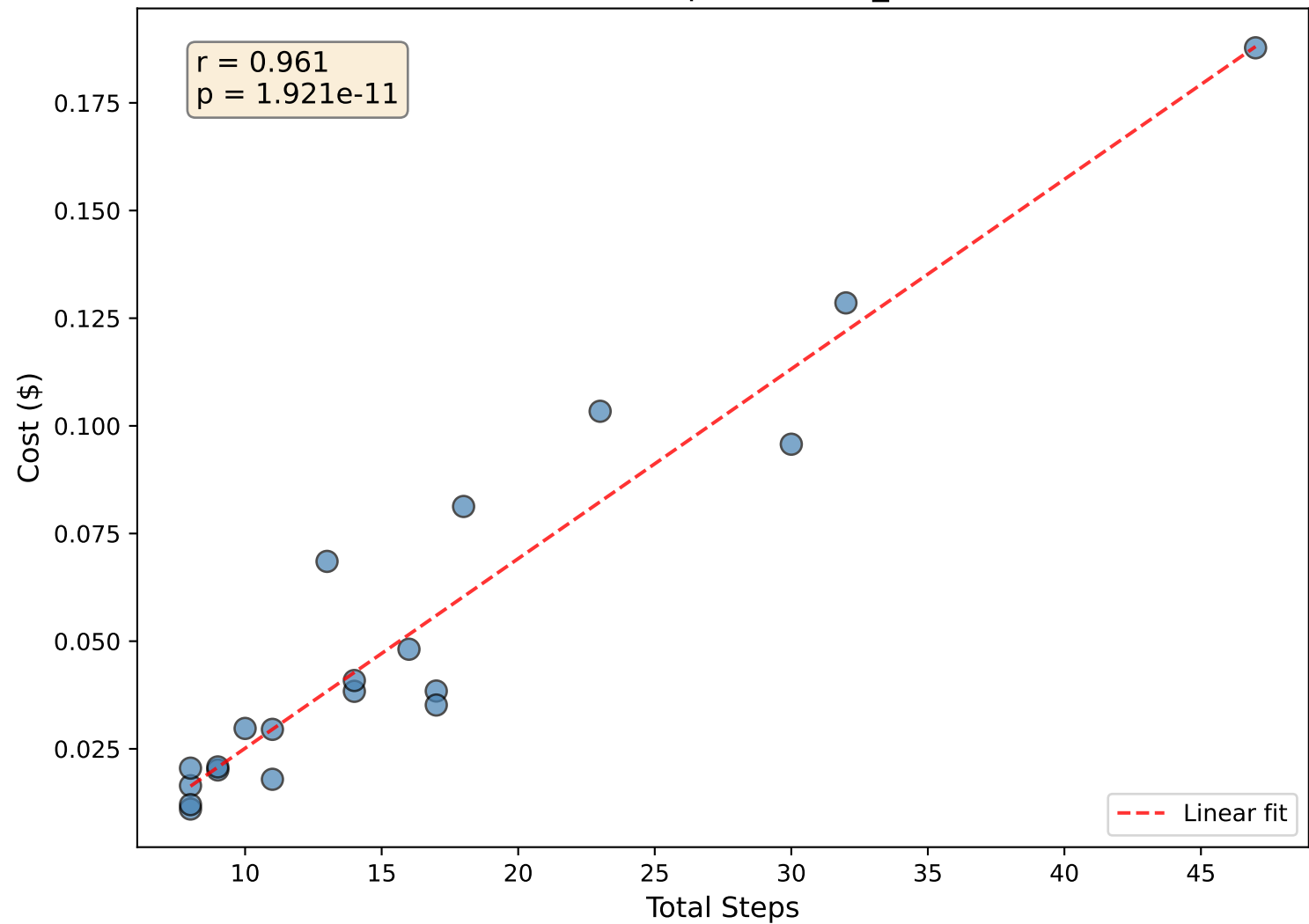
Cost vs Steps (verified_20)
