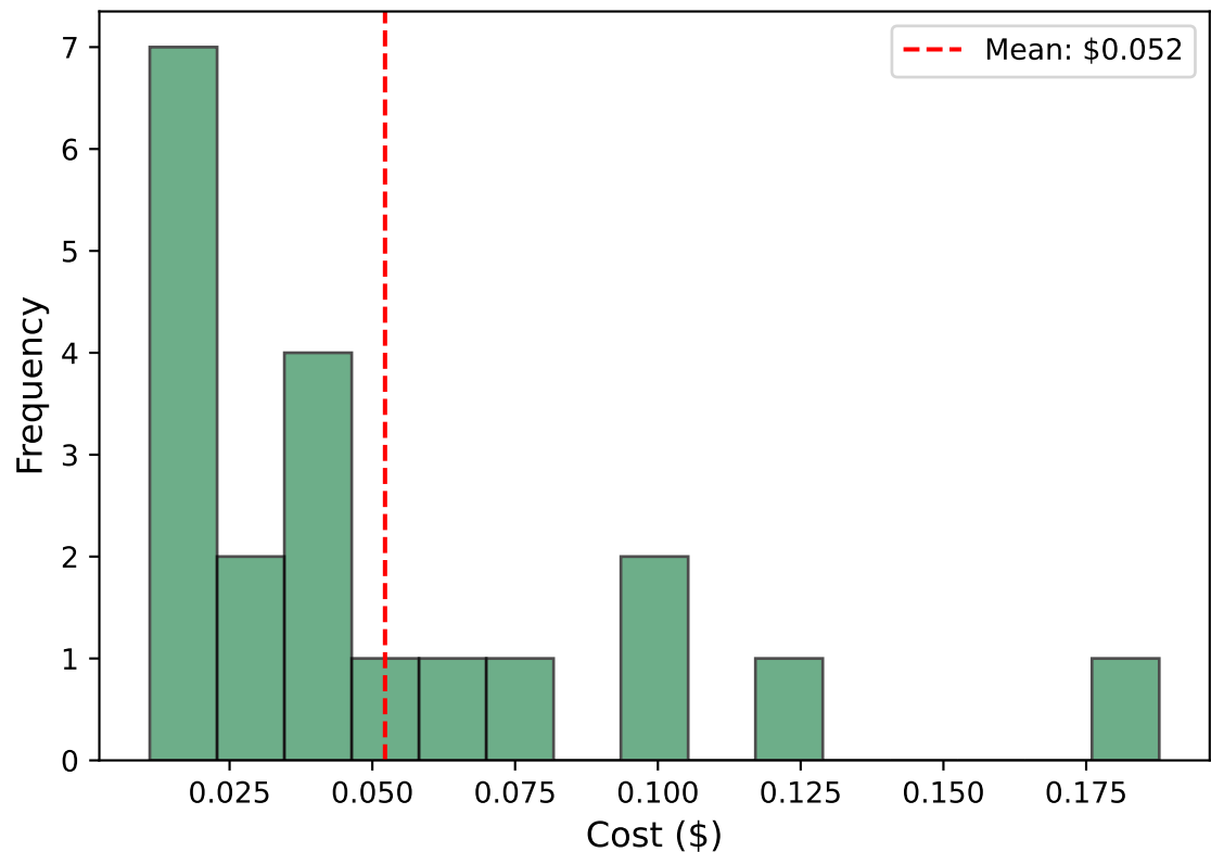
Distribution of Instance Cost
