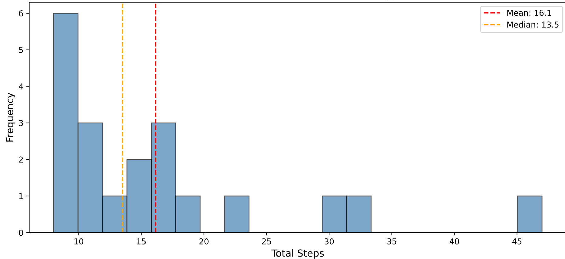
Distribution of Agent Steps (verified_20)
