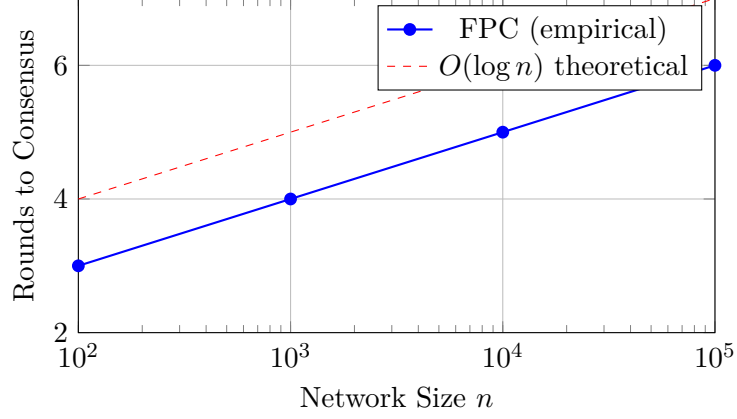
Figure 3: Logarithmic scaling of FPC with network size
