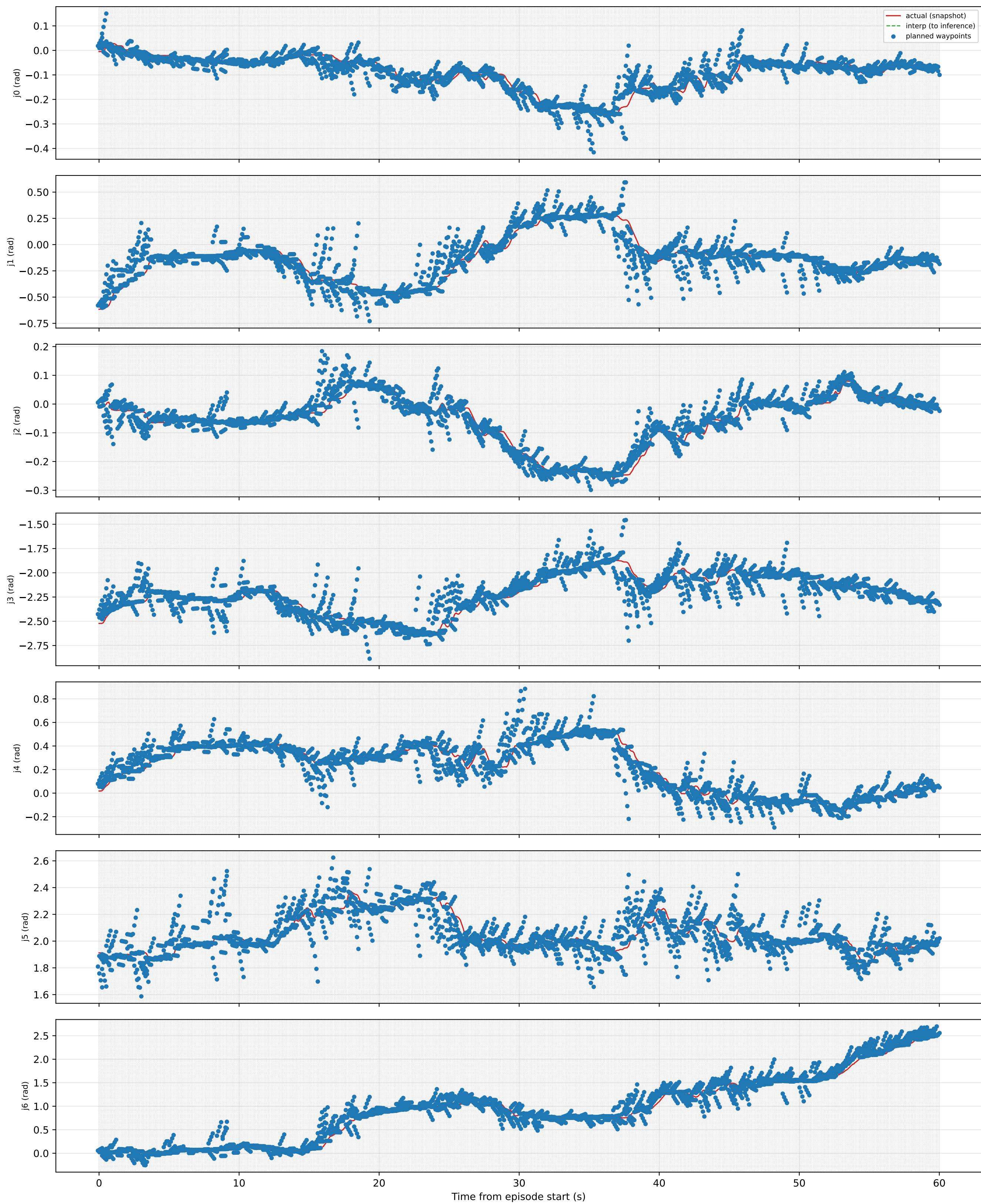
Fig 1: Joint Trajectory — Planned vs Actual
