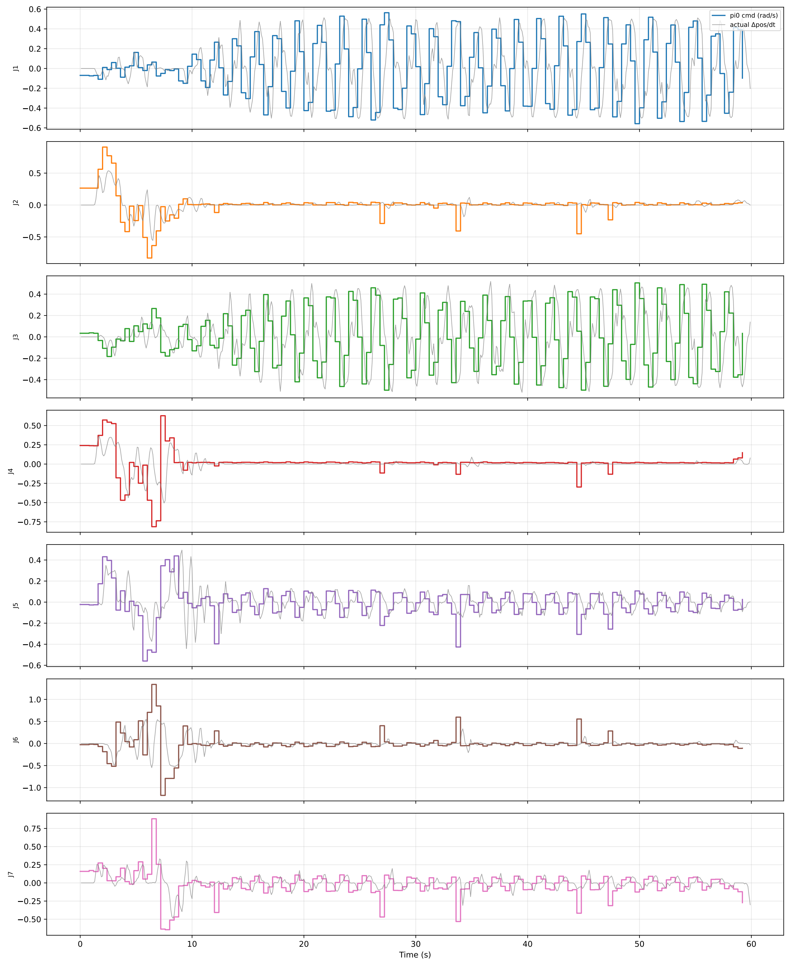
Joint velocity: pi0 commanded ( \times \max_{\Delta} ) vs observed
