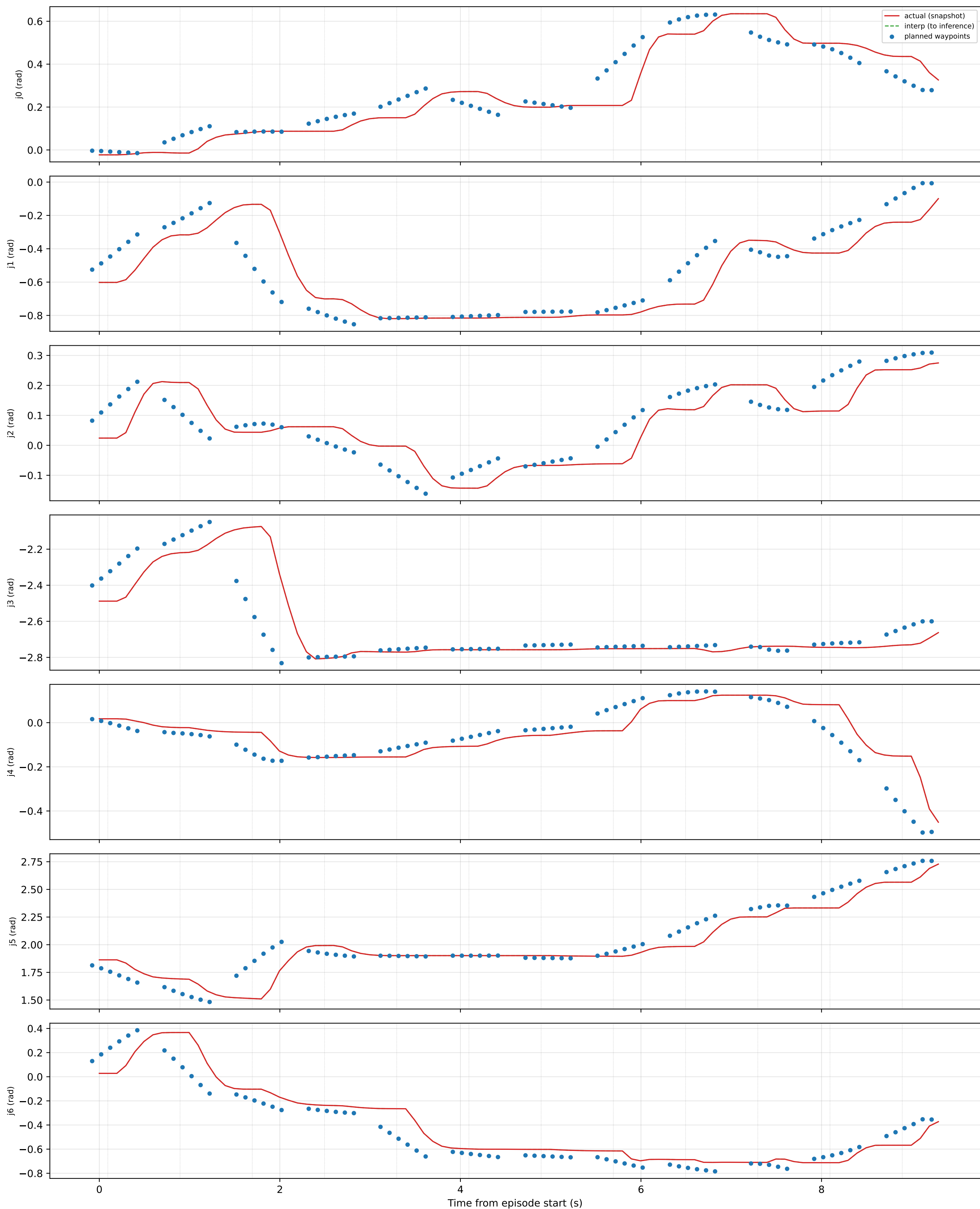
Fig 1: Joint Trajectory — Planned vs Actual
