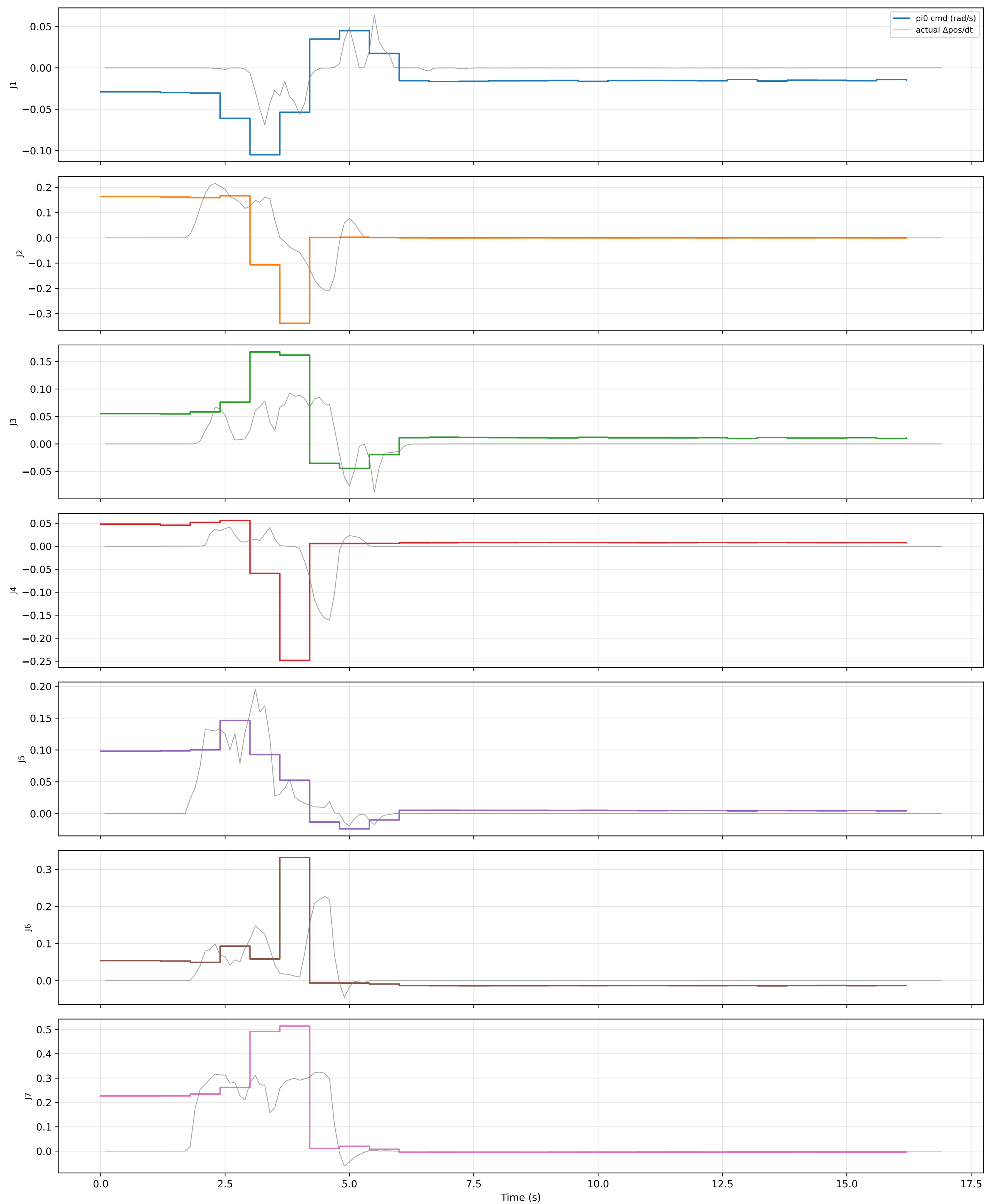
Joint velocity: pi0 commanded ( \times \text{max\_}\Delta ) vs observed
