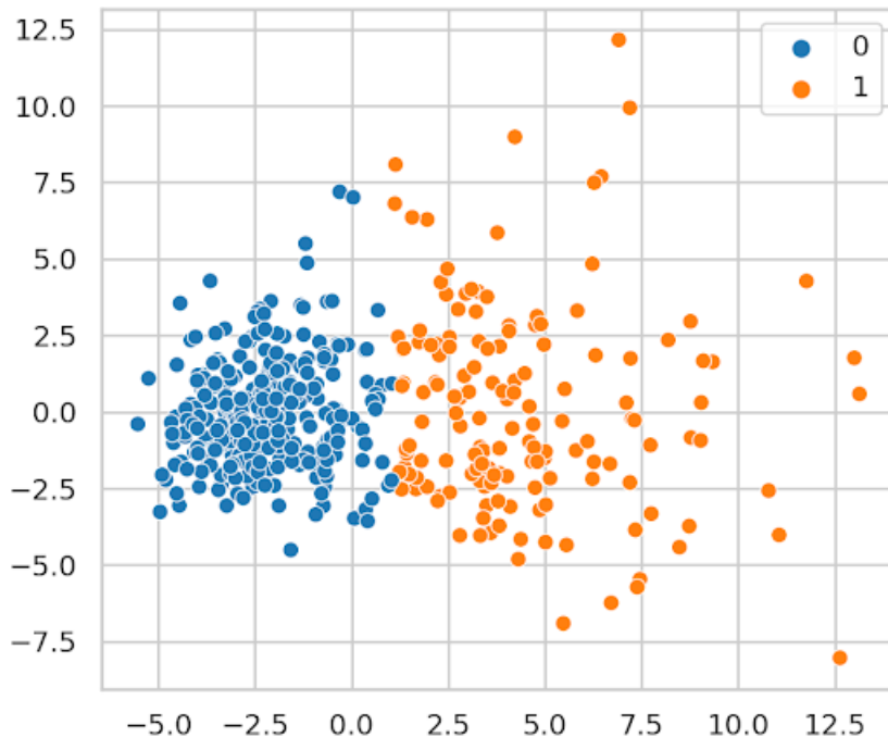
K-Means (Centroides)
