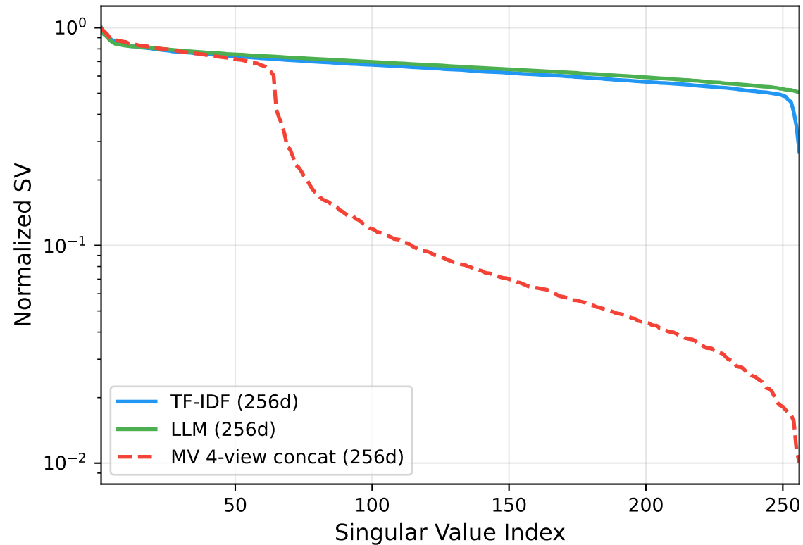
(a) Singular Value Spectrum
