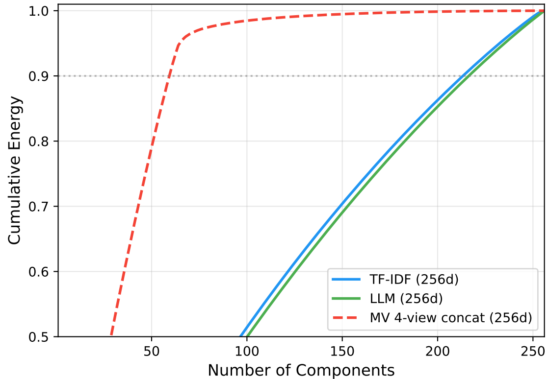
(b) Cumulative Energy
