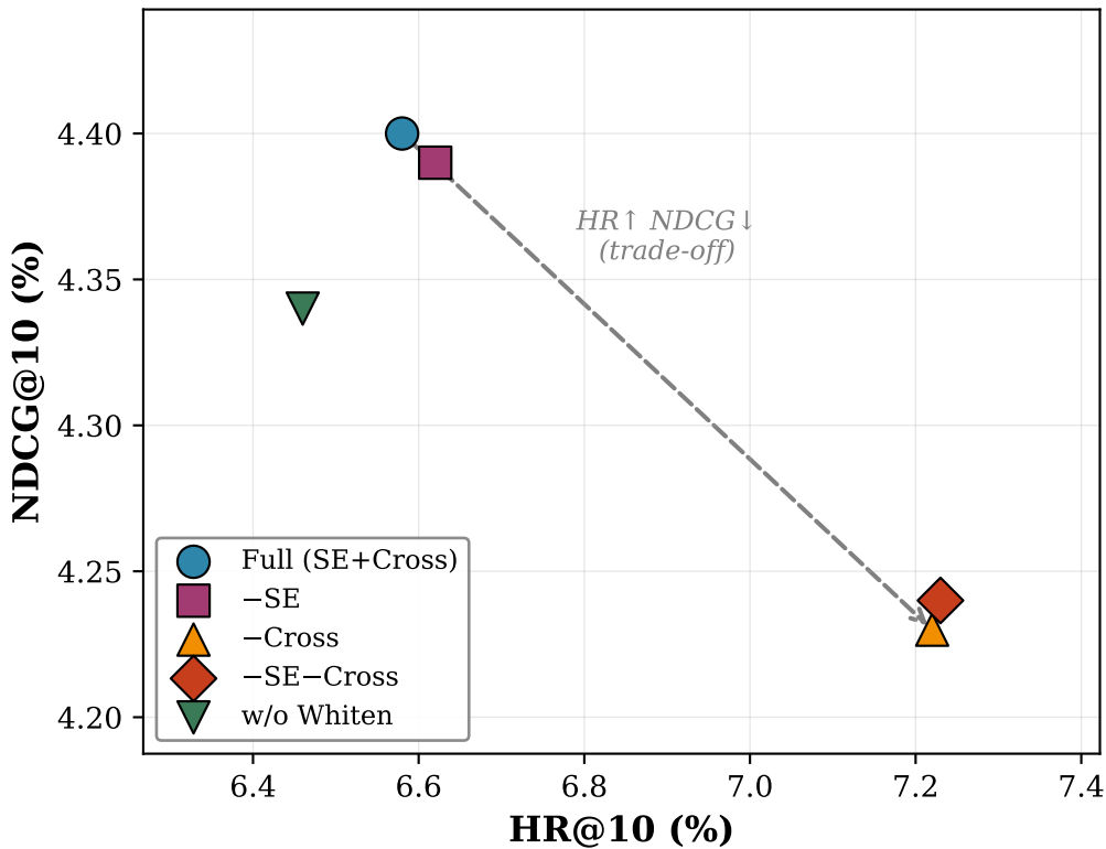
HR-NDCG Trade-off on Toys&Games (7B)
