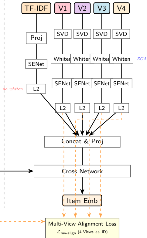
(b) Multi-View
