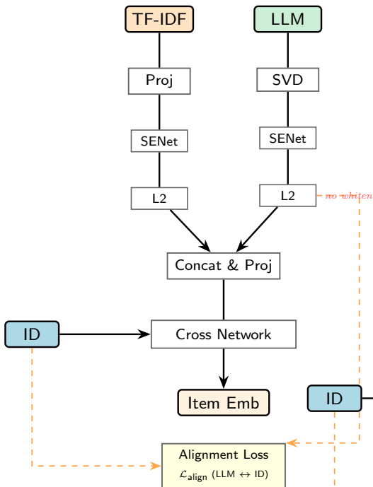
(a) Single-View
