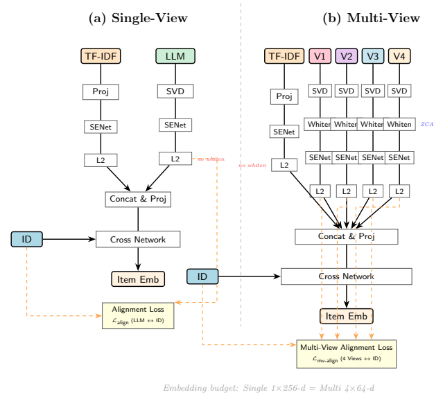
Figure 1: Framework overview of single-view and multi-view architectures. (a) Single-view uses one LLM embedding with L2 normalization. (b) Multi-view uses four prompt perspectives with per-view whitening and multi-view alignment via InfoNCE loss.
