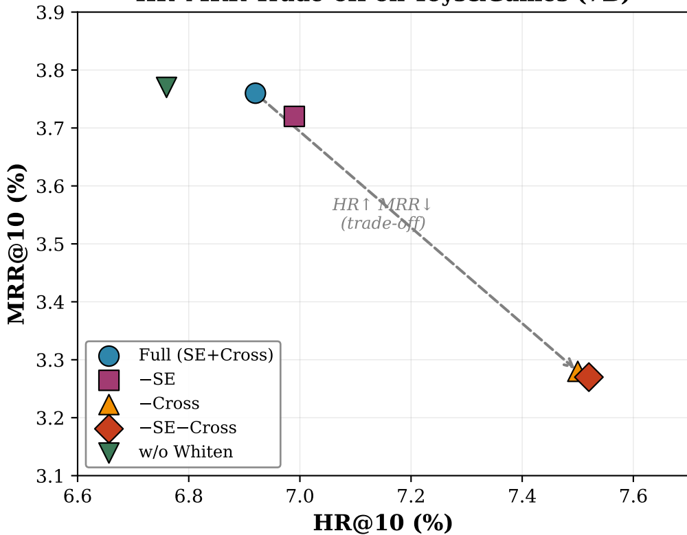
HR-MRR Trade-off on Toys&Games (7B)
