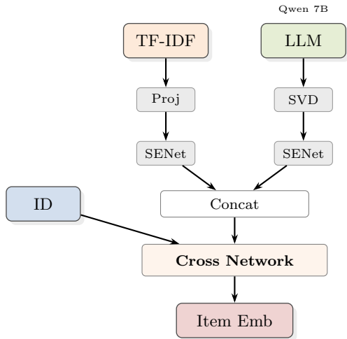
(a) Single-view
