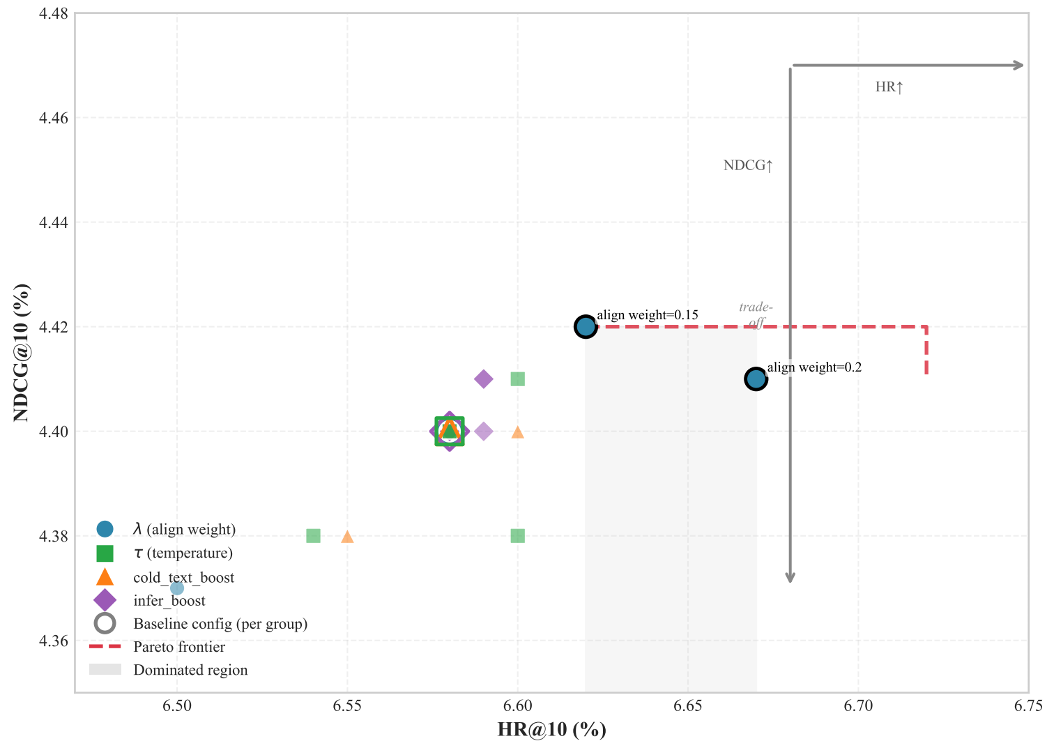
HR@10 vs NDCG@10 Trade-off: Pareto Frontier across Hyperparameter Configs
