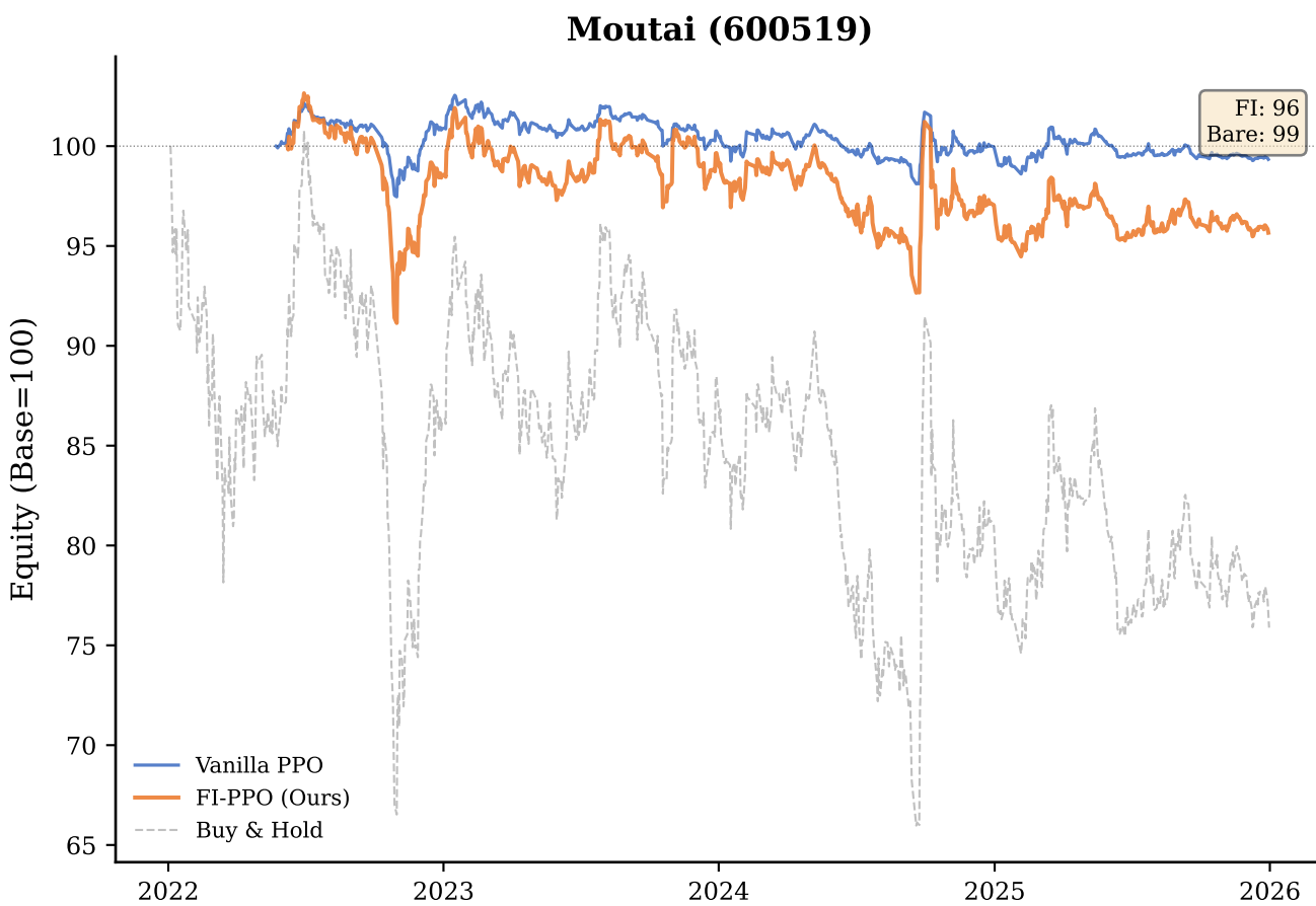
Figure 9: Equity Curves — FI-PPO vs Vanilla PPO vs Buy & Hold (2022-2025)
