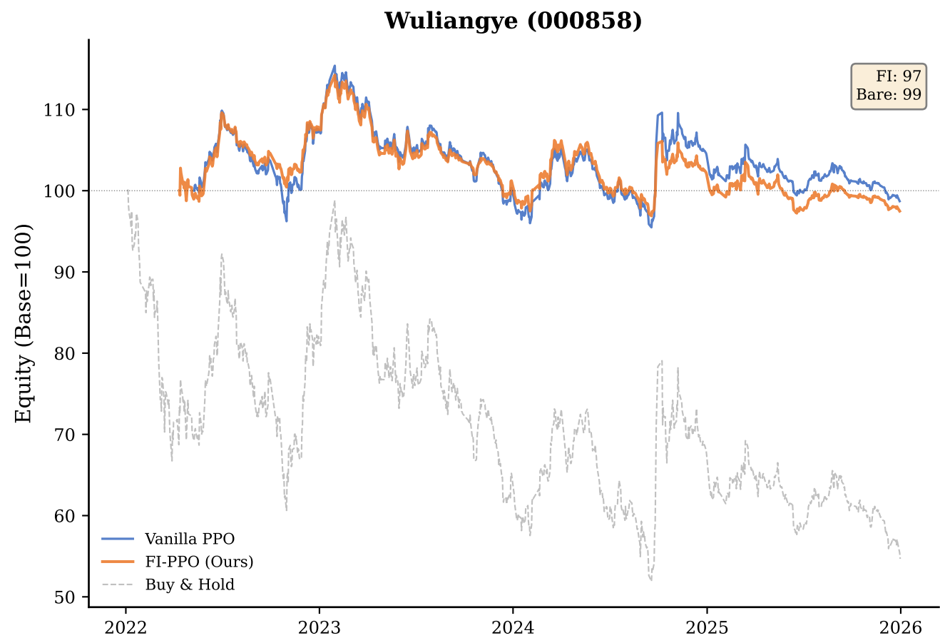
Figure 9: Equity Curves — FI-PPO vs Vanilla PPO vs Buy & Hold (2022-2025)
