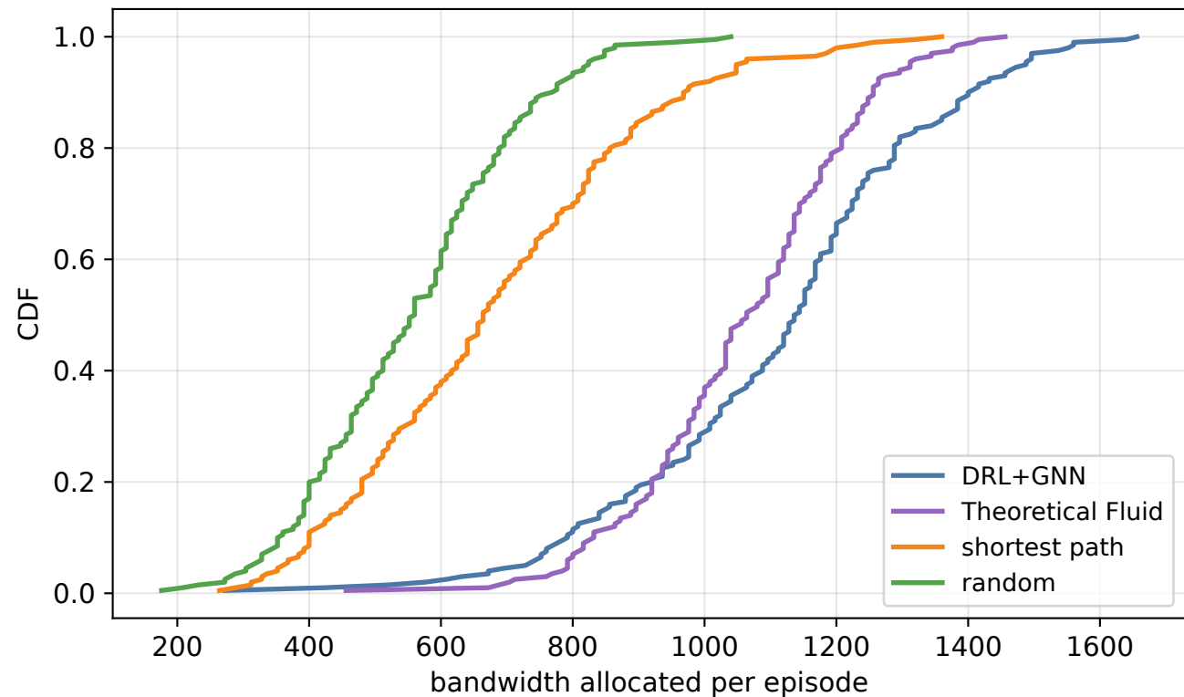
NSFNet ckpt → GEANT2 (200 episodes)
