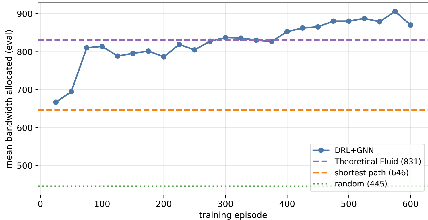
DRL+GNN training on NSFNet
