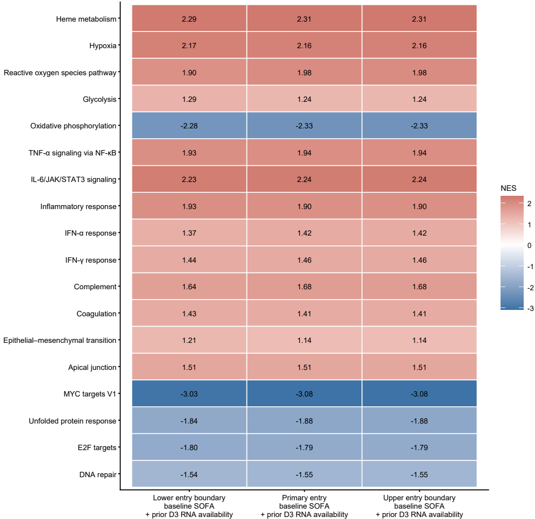
D5 entry-boundary sensitivity
