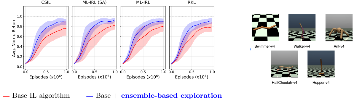
Figure 2: Continuous control imitation learning experiments, results averaged across the 5 environments shown on the right. For any base IL algorithm considered (CSIL Watson et al. [2023] , RKL Ni et al. [2021] , ML-IRL Zeng et al. [2022] ) injecting exploration in the policy updates via critics ensembles leads to faster learning.
