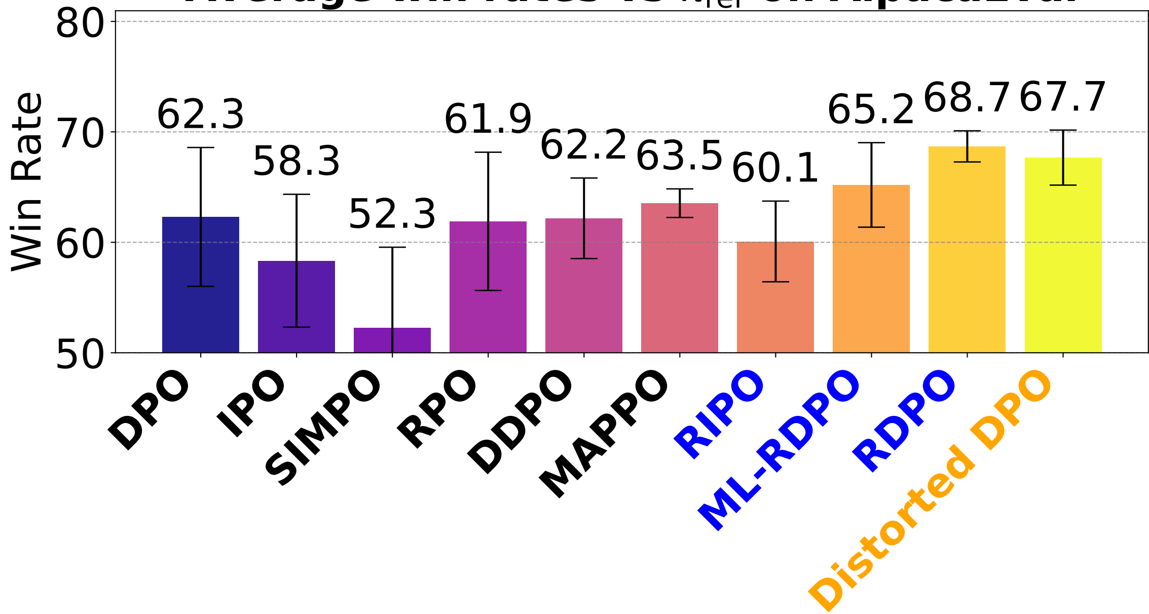
Average win rates vs \pi_{\text{ref}} on AlpacaEval
