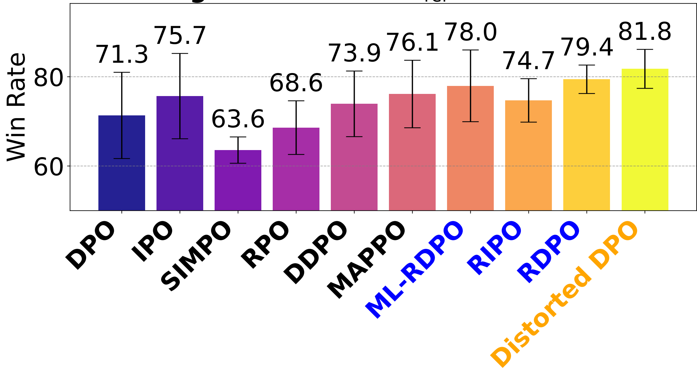
Average win rates vs \pi_{\text{ref}} on Arena Hard
