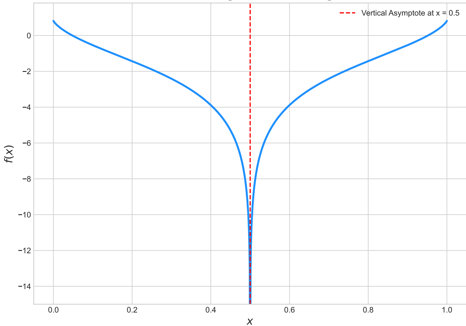
Plot of f(x) = \sigma^{-1}(x \log(2x) + (1-x) \log(2(1-x)))
