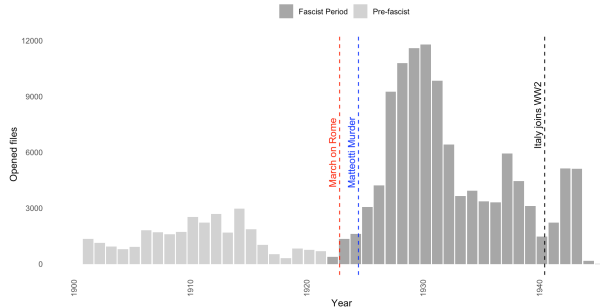
Figure 11: Surveillance Records
