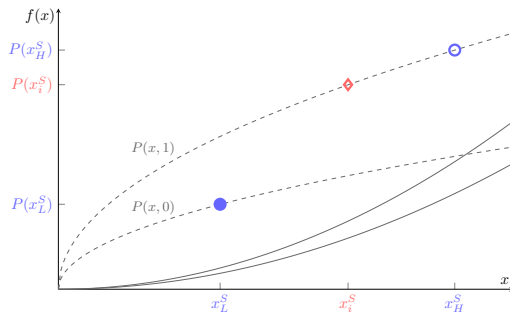
Figure 4: Signalling Equilibrium
