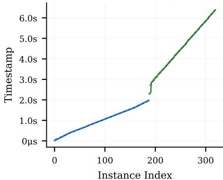
ColumnParallelLinear (320 instances, 2 segments)
