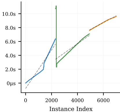
view (7,360 instances)
