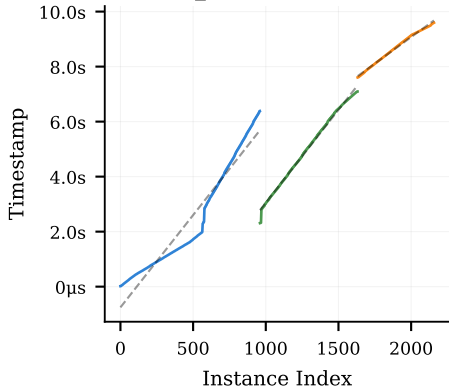
add_ (2,272 instances)
