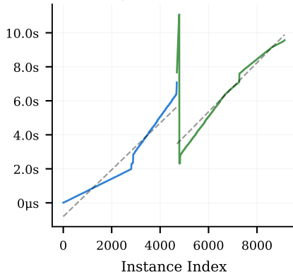
empty (9,625 instances)
