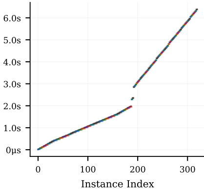
ColumnParallelLinear (LLaMA) (320 inst, 103 segs)
