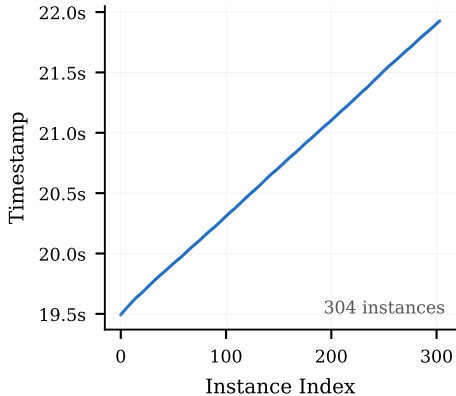
FusedAdam (Qwen3 training, Ascend NPU)
