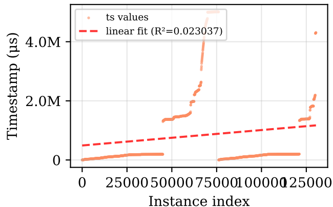
<built-in method get of dic...> (85,343 instances)
