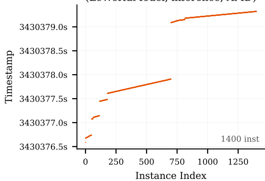
LayerNorm kernel (LeWorldModel, inference, AMD)
