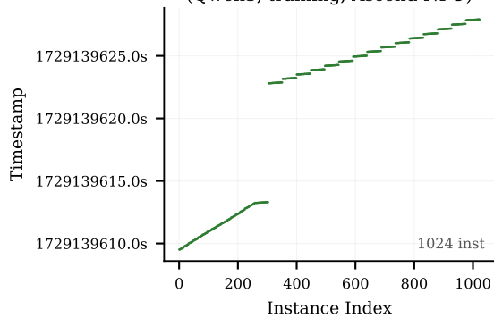
supa_out matmul (Qwen3, training, Ascend NPU)
