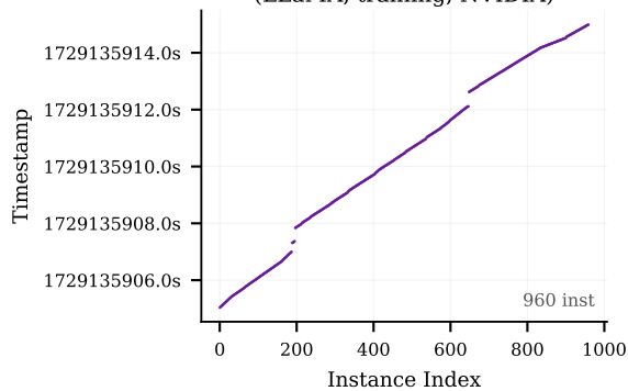
ColumnParallelLinear (LLaMA, training, NVIDIA)
