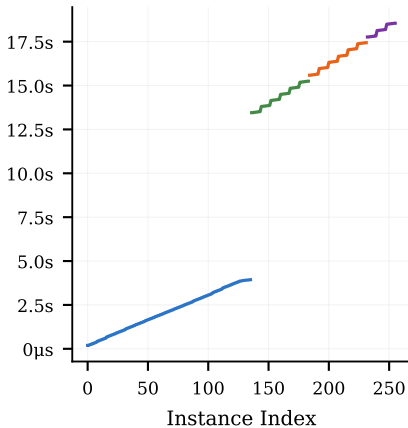
FusedMLP (256 inst)
