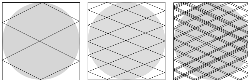
FIGURE 4.4.3. The trajectory with slope 2/5 , at center, visits more of the square than the trajectory with slope 1/2 , at left. The slope of the trajectory at right closely approximates an irrational number; if allowed to continue, this trajectory would visit nearly every part of the square. (The square would soon become black.)
