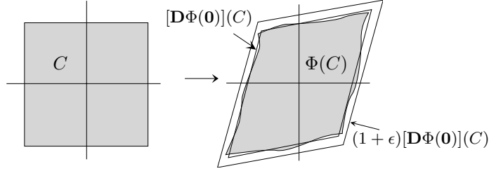
FIGURE A19.3. The cube C is mapped to \Phi(C) , which is almost [\mathbf{D}\Phi(\mathbf{0})](C) , and definitely inside (1+\epsilon)[\mathbf{D}\Phi(\mathbf{0})](C) . As \epsilon \rightarrow 0 , the image \Phi(C) becomes more and more exactly the parallelepiped [\mathbf{D}\Phi(\mathbf{0})]C .
