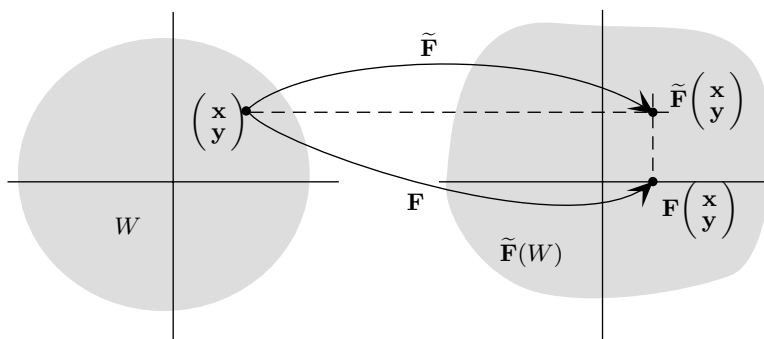
FIGURE A8.1. The mapping \tilde{\mathbf{F}} is designed to add dimensions to the image of \mathbf{F} so that the image has the same dimension as the domain. Here, n = 2 and k = n - k = 1 ; \mathbf{F} maps \left(\begin{smallmatrix} \mathbf{x} \\ \mathbf{y} \end{smallmatrix}\right) to a point in \mathbb{R} , while \tilde{\mathbf{F}} maps it to a point in \mathbb{R}^2 .
