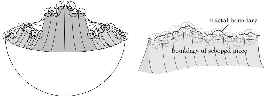
FIGURE 6.10.7. LEFT: We saw this piece-with-complicated-boundary in Figure 6.6.1; its boundary includes a Koch snowflake, with all its fractal complexity. “Scooping out” balls B_i as described in Proposition 6.10.10 turns the piece-with-complicated-boundary into a piece-with-corners (above, the top three scoops have been removed). RIGHT: A closeup of the fractal boundary and the boundary of the scooped piece.
