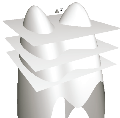
FIGURE 3.1.11. The surface that is the graph of F\left(\begin{smallmatrix} x \\ y \end{smallmatrix}\right) = x^2 - 0.2x^4 - y^2 is sliced horizontally by setting z equal to three different constants. The intersection of the surface and the plane z = c used to slice it is known as a level set or level curve . This intersection is the same as the locus of equation F\left(\begin{smallmatrix} x \\ y \end{smallmatrix}\right) = c .
