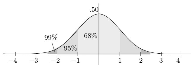
FIGURE 4.2.5. For the normal distribution, 68% of the probability is within one standard deviation; 95% is within two standard deviations; 99% is within 2.5 standard deviations.
