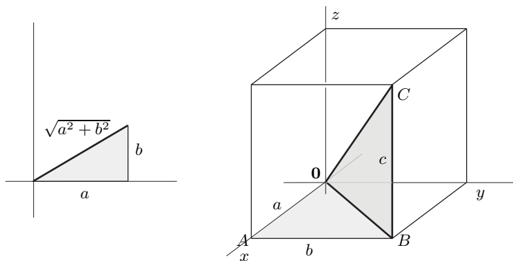
FIGURE 1.4.1. In the plane, the length of the vector with coordinates (a, b) is the ordinary distance from \mathbf{0} to the point \begin{pmatrix} a \\ b \end{pmatrix} . In space, the length of the vector from \mathbf{0} to C is the ordinary distance between \mathbf{0} and C : \mathbf{OBC} is a right triangle, the distance from \mathbf{0} to B is \sqrt{a^2 + b^2} (applying the Pythagorean theorem to the pale triangle), and the distance from B to C is c , so (applying the Pythagorean theorem to the darker triangle) the distance from \mathbf{0} to C is \sqrt{a^2 + b^2 + c^2} .
