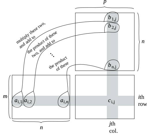
FIGURE 1.2.1. The entry c_{i,j} of the matrix C = AB is the sum of the products of the entries a_{i,k} of the matrix A and the corresponding entry b_{k,j} of the matrix B . The entries a_{i,k} are all in the i th row of A ; the first index i is constant, and the second index k varies. The entries b_{k,j} are all in the j th column of B ; the first index k varies, and the second index j is constant. Since the width of A equals the height of B , the entries of A and those of B can be paired up exactly.
