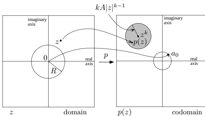
FIGURE 1.6.8. If |z| \geq R , the complex number p(z) is in the shaded disc of radius kA|z|^{k-1} around z^k , since
