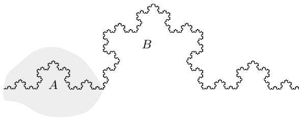
FIGURE 5.5.3. The curve B consists of four copies of A . It is also A scaled up by a factor of 3. It is the difference between these factors 3 and 4 that results in the fractional dimension of the curve.
