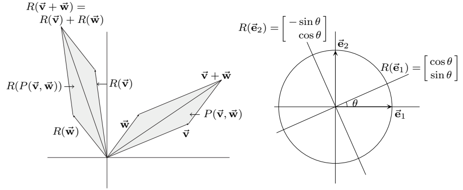
FIGURE 1.3.10. Figure for Example 1.3.9. LEFT: The sum of the rotations is the rotation of the sum. Rather than rotating the vectors \vec{v} and \vec{w} , we rotate the whole parallelogram P(\vec{v}, \vec{w}) that they span (the parallelogram with sides \vec{v} and \vec{w} ). Then R(P(\vec{v}, \vec{w})) is the parallelogram spanned by R(\vec{v}), R(\vec{w}) , and the diagonal of R(P(\vec{v}, \vec{w})) is R(\vec{v} + \vec{w}) . It is also true that R(c\vec{v}) = cR(\vec{v}) , so rotation is linear. RIGHT: We see that the matrix of the transformation R giving rotation by \theta counterclockwise around the origin is \begin{bmatrix} \cos \theta & -\sin \theta \\ \sin \theta & \cos \theta \end{bmatrix} .
