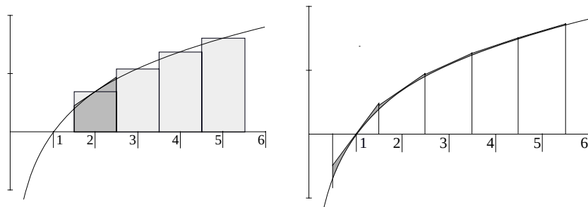
FIGURE A16.1. LEFT: The sum \ln 1 + \ln 2 + \cdots + \ln n is a midpoint Riemann sum for the integral \int_{1/2}^{n+1/2} \ln x \, dx . The k th rectangle has the same area as the trapezoid whose top edge is tangent to the graph of \ln x at \ln n , as illustrated when k = 2 . RIGHT: The difference between the areas of the trapezoids and the area under the graph of the logarithm is the shaded region. It has finite total area, as shown in equation A16.3.
