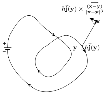
FIGURE 6.12.5. The cross product
