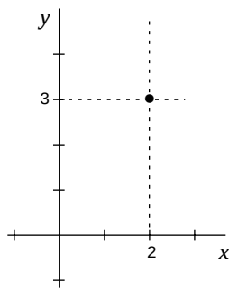
FIGURE 1.1.1. The point \begin{pmatrix} 2 \\ 3 \end{pmatrix} .
