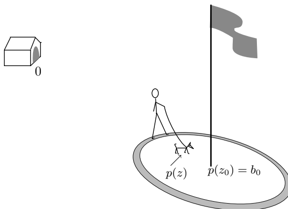
FIGURE 1.6.9. We have shown that there is a point z_0 at which |p| has a minimum. We assume that p(z_0) \neq 0 and show a contradiction: if |u| is small, the leash is shorter than the radius |b_j| r^j of the circle on which the man is walking, so at some point the dog will be closer to the doghouse than the distance from flagpole to doghouse: |p(z)| < |p(z_0)| . Since |p| has a minimum at z_0 , this is impossible, so our assumption p(z_0) \neq 0 is false.
