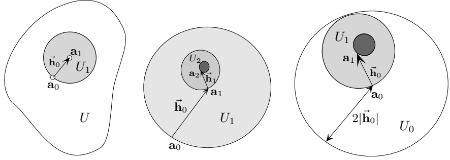
FIGURE 2.8.7. Equation 2.8.51 defines the neighborhood U_1 for which Newton's method is guaranteed to work when inequality 2.8.53 is satisfied. LEFT: the neighborhood U_1 is the ball of radius |\vec{h}_0| = |\mathbf{a}_1 - \mathbf{a}_0| around \mathbf{a}_1 , so \mathbf{a}_0 is on the border of U_1 . MIDDLE: a blow-up of U_1 (shaded), showing the neighborhoods U_2 (dark) and U_3 (darker). RIGHT: The ball U_0 described in Proposition 2.8.14.
