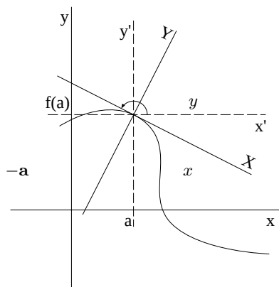
FIGURE 3.9.3 In the coordinates X, Y centered at \begin{pmatrix} a \\ f(a) \end{pmatrix} , the curve of equation y = f(x) is the curve of equation Y = g(X) , where the Taylor polynomial of g starts with quadratic terms.
