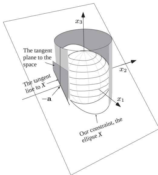
FIGURE 3.7.3 The point -\mathbf{a} is a minimum of the function
