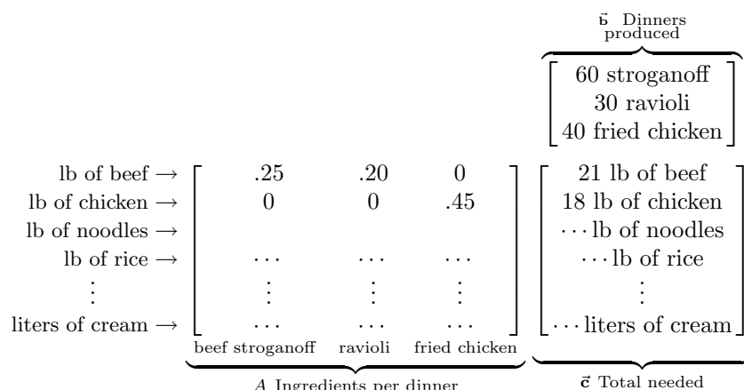
FIGURE 1.3.1. The matrix A is the transformation associating the number of dinners of various sorts produced to the total ingredients needed. \triangle
