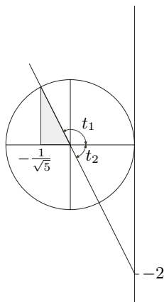
FIGURE 2.9.2. The diagram for Example 2.9.9.
