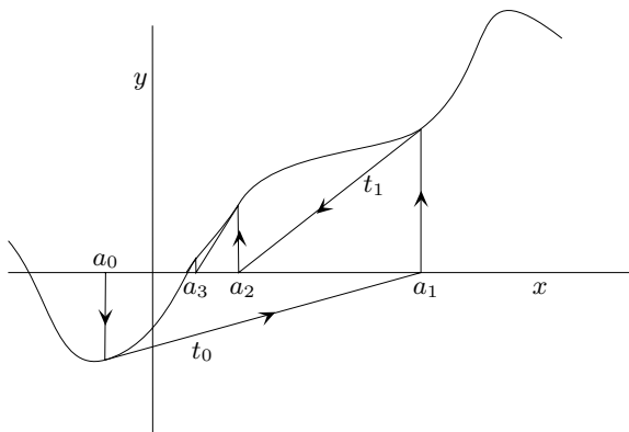
FIGURE 2.8.2. Newton's method: We start with a_0 , and draw the tangent to the curve at the point with x -coordinate a_0 . The point where that tangent t_0 intersects the x -axis is a_1 . Now we draw the tangent to the curve at the point with x -coordinate a_1 . That tangent t_1 intersects the x -axis at a_2 \dots . Each time we calculate a_{n+1} from a_n we are calculating the intersection with the x -axis of the line tangent to the curve at the point with x -coordinate a_n .
