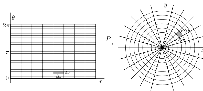
FIGURE 4.10.1. The polar coordinate map P maps the rectangle at left, with dimensions \Delta r and \Delta\theta , to the curvilinear box at right, with two straight sides of length \Delta r and two curved sides measuring r\Delta\theta (for different values of r ).
