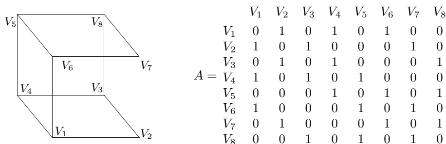
FIGURE 1.2.6. LEFT: The graph of a cube. RIGHT: Its adjacency matrix A . If vertices V_i and V_j are joined by a single edge, the (i, j) th and (j, i) th entries of the matrix are 1; otherwise they are 0.
