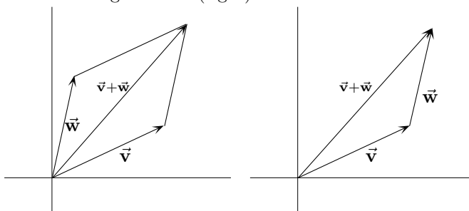
FIGURE 1.1.4. In the plane, the sum \vec{v} + \vec{w} is the diagonal of the parallelogram at left. We can also add them by putting them head to tail.
