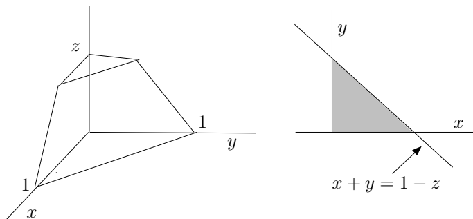
FIGURE 4.5.6. LEFT: The pyramid of Figure 4.5.5, truncated at height z . RIGHT: The plane at height z , put flat.
