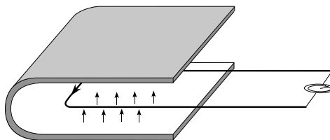
FIGURE 6.12.6. A loop of wire is inserted in the magnetic field due to a permanent U-shaped magnet. Outside the magnet the wire is connected to an ammeter. If the wire is pulled out of the magnet, the charges in the piece of wire transverse to the motion are “pushed” by the Lorentz force \frac{\vec{\mathbf{v}}}{c} \times \vec{\mathbf{B}} , in the direction indicated by the arrow.
