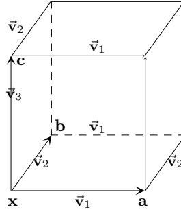
FIGURE 6.6.14 The cube spanned by the vectors \vec{v}_1, \vec{v}_2, \vec{v}_3 , anchored at \mathbf{x} . To lighten notation set \mathbf{a} = \mathbf{x} + \vec{v}_1 , \mathbf{b} = \mathbf{x} + \vec{v}_2 , and \mathbf{c} = \mathbf{x} + \vec{v}_3 . The original three vectors are drawn in dark lines; the translates in lighter or dotted lines.
