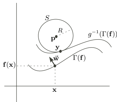
FIGURE A23.2. The moved graph g^{-1}(\Gamma(\mathbf{f})) fails to be transversal to the sphere S (here a circle) if there is a point \mathbf{y} = g^{-1}\left(\begin{smallmatrix} \mathbf{x} \\ \mathbf{f}(\mathbf{x}) \end{smallmatrix}\right) and a unit vector \vec{\mathbf{w}} orthogonal to \Gamma(\mathbf{f}) at \left(\begin{smallmatrix} \mathbf{x} \\ \mathbf{f}(\mathbf{x}) \end{smallmatrix}\right) such that R\vec{\mathbf{w}} = [\mathbf{D}g](\mathbf{y} - \mathbf{p}) .
