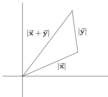
FIGURE 1.4.7. The triangle inequality: |\vec{x} + \vec{y}| < |\vec{x}| + |\vec{y}| .
