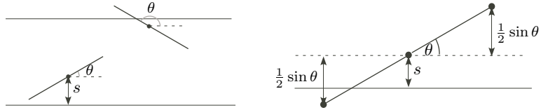
FIGURE 4.2.3. LEFT: The position of a needle is encoded by the distance s \in [0, 1/2] from the center of a needle to the nearest line and the angle \theta \in [0, \pi) that the needle makes with the horizontal. RIGHT: The needle will intersect a line if s < \frac{1}{2} \sin \theta .
