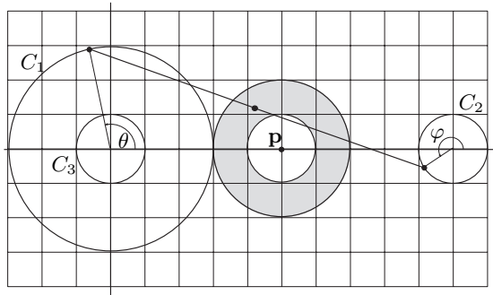
FIGURE 2.10.5. Above, C_1 is the circle of radius 3 centered at the origin, and C_2 is the circle of radius 1 centered at \begin{pmatrix} 10 \\ 0 \end{pmatrix} . The midpoint of every line segment connecting a point in C_1 to a point in C_2 lies in the annular region between the circles of radius 2 and 1 centered at \mathbf{p} . One such midpoint is shown. Extending the line segment to the far side of C_2 would give a different midpoint.
