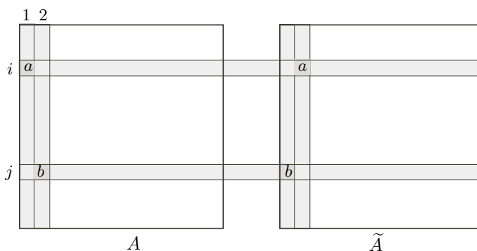
FIGURE 4.8.1. In both matrices, C is the unshaded part. LEFT: The n \times n matrix A , the i th and j th row and the first two columns shaded. RIGHT: The matrix \tilde{A} , identical to A except that the first two columns are exchanged. Let a, b be the shaded entries a = a_{i,1} = \tilde{a}_{i,2} and b = a_{j,2} = \tilde{a}_{j,1} . Note that the unshaded parts coincide: A_{[i,1][j-1,1]} = \tilde{A}_{[j,1][i,1]} .
