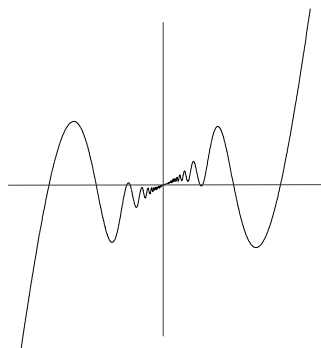
FIGURE 1.9.2. Graph of the function
