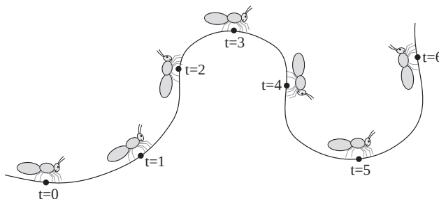
FIGURE 3.1.16. We imagine a parametrized curve as an ant taking a walk in the plane or in space. The parametrization tells where the ant is at any given time.
