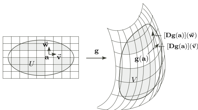
FIGURE 1.7.3. The function \mathbf{g} : \mathbb{R}^2 \rightarrow \mathbb{R}^2 maps a point \mathbf{a} \in U to a point \mathbf{g}(\mathbf{a}) \in V ; in particular, it maps the white cross in U to the deformed cross in V . The derivative of \mathbf{g} at \mathbf{a} maps the vector \vec{\mathbf{v}} anchored at \mathbf{a} to [\mathbf{Dg}(\mathbf{a})](\vec{\mathbf{v}}) , which is anchored at \mathbf{g}(\mathbf{a}) ; it maps the vector \vec{\mathbf{w}} anchored at \mathbf{a} to [\mathbf{Dg}(\mathbf{a})](\vec{\mathbf{w}}) , which is anchored at \mathbf{g}(\mathbf{a}) .
