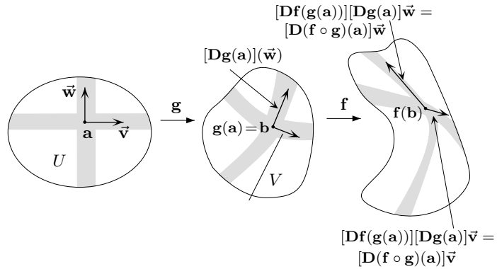
FIGURE 1.8.2. The function \mathbf{g} maps a point \mathbf{a} \in U to a point \mathbf{g}(\mathbf{a}) \in V . The function \mathbf{f} maps the point \mathbf{g}(\mathbf{a}) = \mathbf{b} to the point \mathbf{f}(\mathbf{b}) . The derivative of \mathbf{g} maps the vector \vec{v} to [Dg(\mathbf{a})](\vec{v}) . The derivative of \mathbf{f} \circ \mathbf{g} maps \vec{v} to [Df(\mathbf{g}(\mathbf{a}))][Dg(\mathbf{a})]\vec{v} , which, of course, is identical to [Df(\mathbf{g}(\mathbf{a}))][Dg(\mathbf{a})]\vec{v} .
