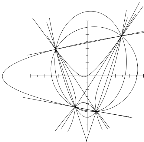
FIGURE A2.7.3. The curves f_m \left( \frac{x}{y} \right) = y^2 + qx + r - \frac{p^2}{4} + m(x^2 - y + p/2) = 0 for seven different values of m .
