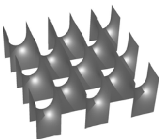
FIGURE FOR EXERCISE 3.27. Scherk's surface, of equation
