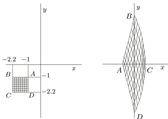
FIGURE 2.10.4. The function \mathbf{f} of Example 2.10.5 maps the region at left to the region at right. In this region, \mathbf{f} is invertible.
