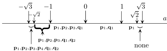
FIGURE 3.7.8. As a decreases from \sqrt{3} to -\sqrt{3} , the set X_a grows; when a \in (\sqrt{2}, \sqrt{3}) , it contains none of the \mathbf{p}_i, \mathbf{q}_i , and when a \in (-\sqrt{2}, -\sqrt{3}) , it contains them all.
