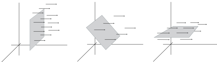
FIGURE 6.5.3. The flow of \vec{F} through a surface depends on the angle between \vec{F} and the surface. LEFT: \vec{F} is orthogonal to the surface, providing maximum flow. MIDDLE: \vec{F} is not orthogonal to the surface, allowing less flow. RIGHT: \vec{F} is parallel to the surface; the flow through the surface is 0.
