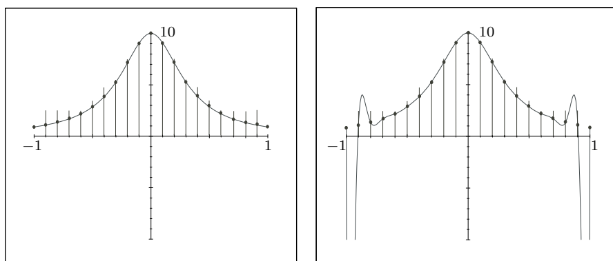
FIGURE 2.5.3. LEFT: The function \frac{1}{x^2 + 1/10} , between x = -1 and x = 1 . RIGHT: The unique polynomial of degree 20 reconstituted from the values of the function at the 21 points -1, -0.9, \dots, 0.9, 1 (the marked dots), using Lagrange interpolation. Near the boundary of the domain of interpolation, Lagrange interpolation is a terrible way to approximate a function.
