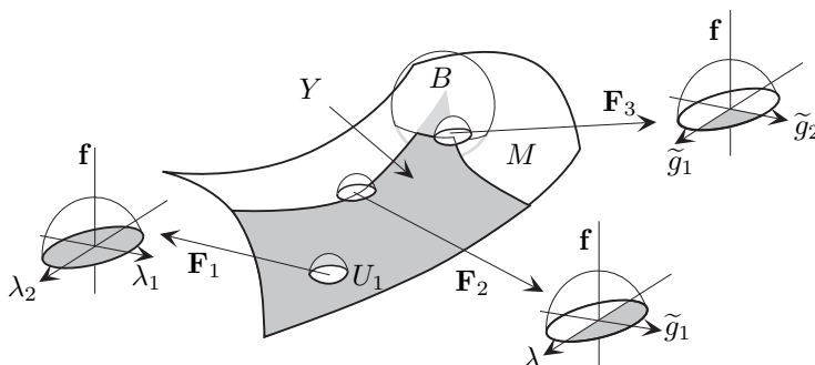
FIGURE 6.10.4. Here, n = 3 and k = 2 . The darkly shaded region is Y , the piece-with-corners. At all points in the manifold M , we have \mathbf{f} = \mathbf{0} , so \mathbf{F} goes from a neighborhood V \subset \mathbb{R}^3 of \mathbf{x} \in Y (more generally, V \subset \mathbb{R}^n ) to a subset of \mathbb{R}^3 , taking M to a neighborhood of \mathbf{0} in the (x, y) -plane (in the general case, to a neighborhood of the origin in a subspace of dimension k , where the other n - k coordinates vanish). Thus \mathbf{F} flattens M and straightens out its boundary. Here we have three instances of the function \mathbf{F} ,
