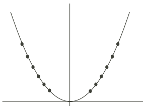
FIGURE 3.8.2 Let S be a collection of points on the parabola y = x^2 , symmetric with respect to the y -axis. The random variables x and y are uncorrelated, even though y = x^2 .
