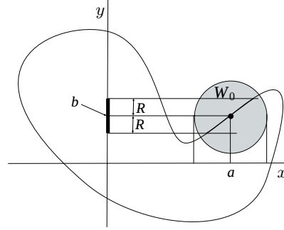
FIGURE 2.10.11. In a neighborhood of \begin{pmatrix} a \\ b \end{pmatrix} the equation F = 0 expresses x implicitly as a function of y . That neighborhood is contained in the ball W_0 of radius r = 2R|L^{-1}| . But the whole curve is not the graph of a function f expressing x as a function of y ; near y = b , there are four such functions.
