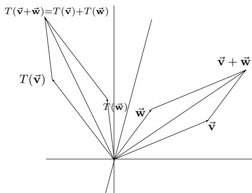
FIGURE 1.3.5. Reflection is linear.
