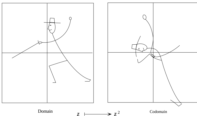
FIGURE 0.7.6. “Graph” of the complex-valued squaring function f(z) = z^2 .
