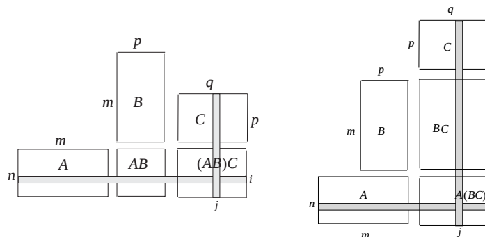
FIGURE 1.2.5. LEFT: This way of writing the matrices corresponds to calculating (AB)C . The i th row of AB depends on the i th row of A and the entire matrix B . RIGHT: This format corresponds to calculating A(BC) . The j th column of BC depends on the j th column of C and the entire matrix B .
