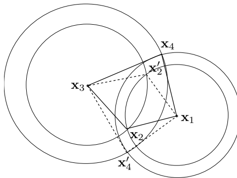
FIGURE 3.1.8. Two possible positions of a linkage with the same \mathbf{x}_1 and \mathbf{x}_3 are shown in solid and dotted lines. The other two are \mathbf{x}_1, \mathbf{x}_2, \mathbf{x}_3, \mathbf{x}'_4 and \mathbf{x}_1, \mathbf{x}'_2, \mathbf{x}_3, \mathbf{x}_4 .
