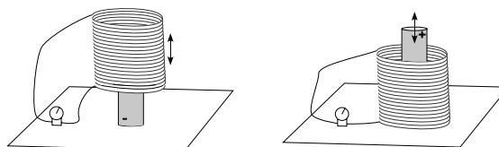
FIGURE 6.12.3. You can put the magnet on the table and jiggle the coil up and down around it (left), or you can put the coil on the table and jiggle the magnet in and out of the coil (right). The result is the same: an alternating current in the coil.
