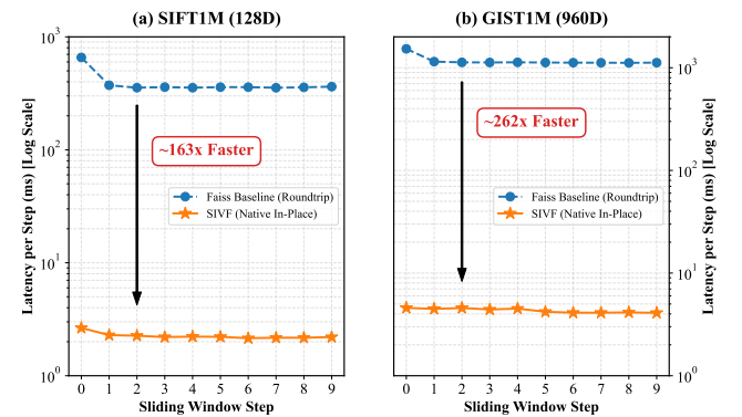
Figure 11: End-to-End Streaming Performance.
