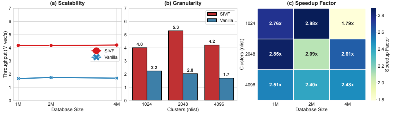
Figure 2: Microbenchmark performance of vector ingestion.
