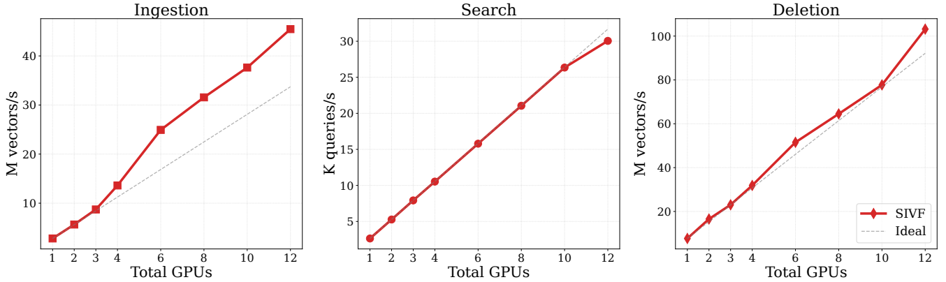
Figure 13: Scalability across a 4-node cluster of 12 GPUs.
