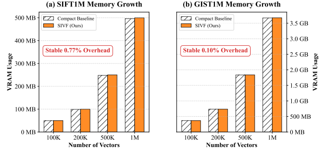
Figure 12: Memory Efficiency and Scalability.
