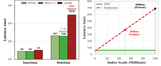
(a) Physical deletion overhead. (b) Tombstone scalability trap.
