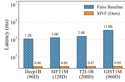
Figure 7: Deletion latency.
