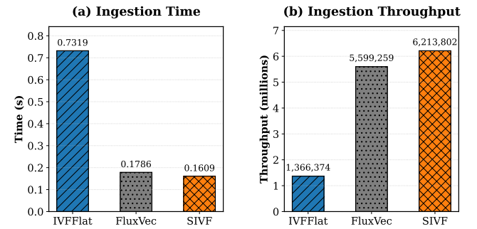
Figure 10: Performance comparison under Zipfian skewed data distribution.
