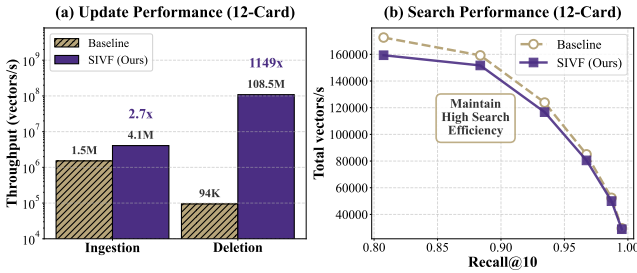
Figure 14: Distributed performance on the 12-GPU cluster (DINO10B dataset).
