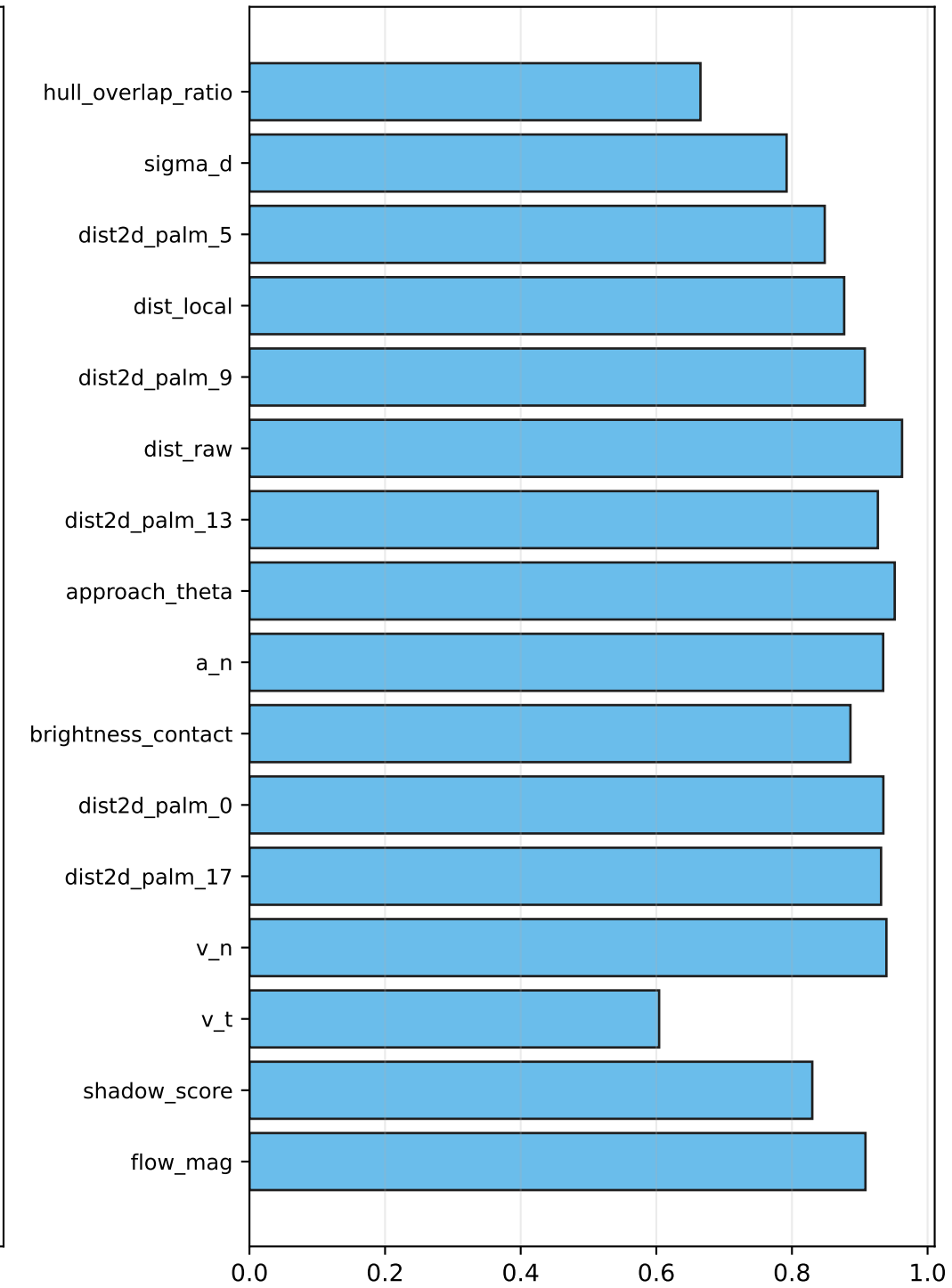
(d) Bhattacharyya overlap
