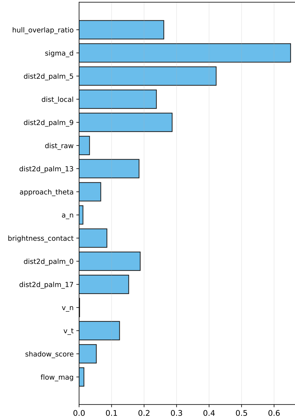
(b) |Cohen's d|
