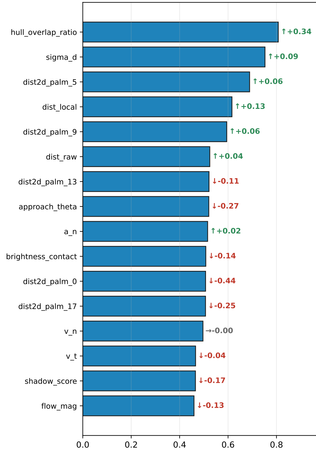
(a) AUROC (5-fold CV LR)
