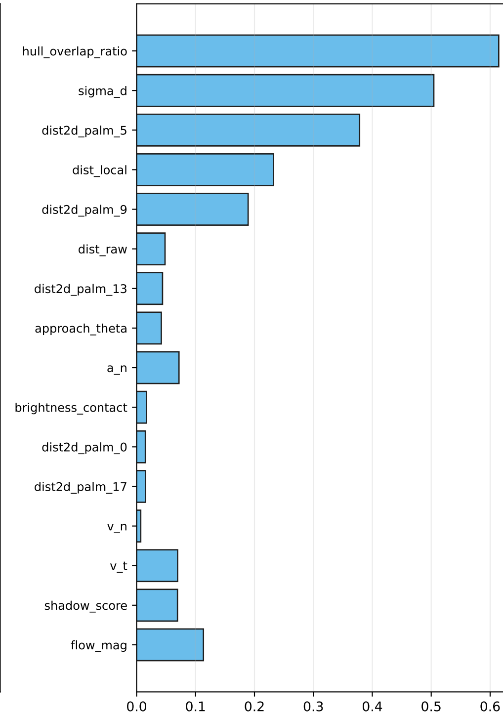
(c) Rank-biserial |r|
