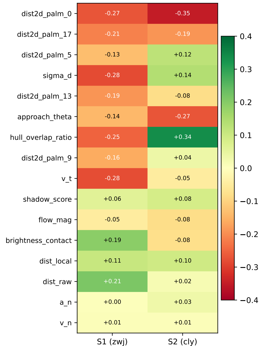
(a) \Delta AUROC (B – A)
