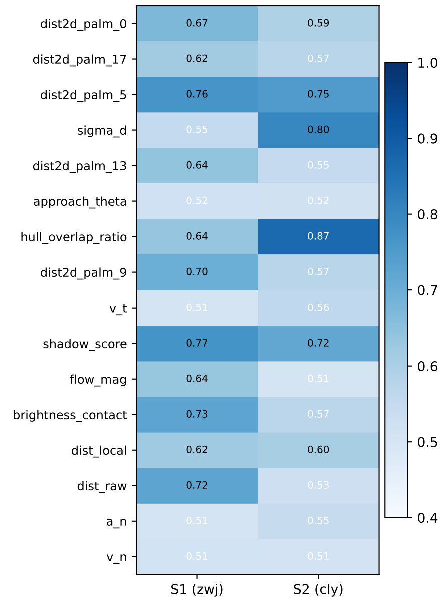
(c) Exp-B AUROC
