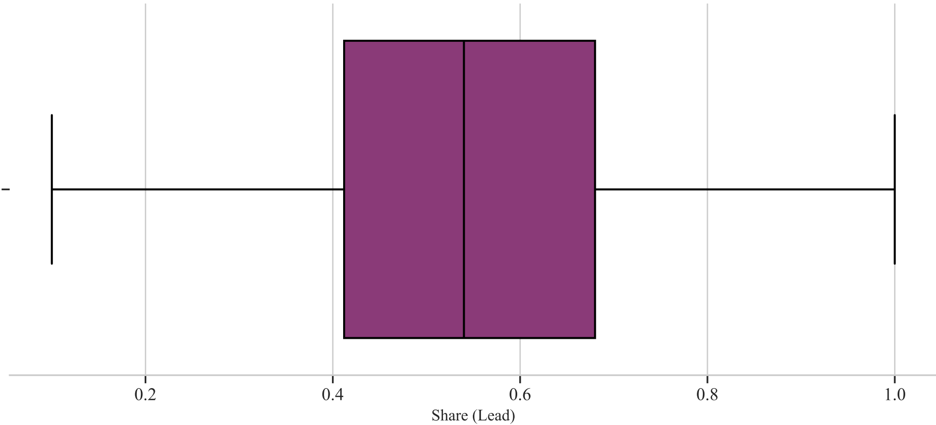
Boxplot for `Share (Lead)`
