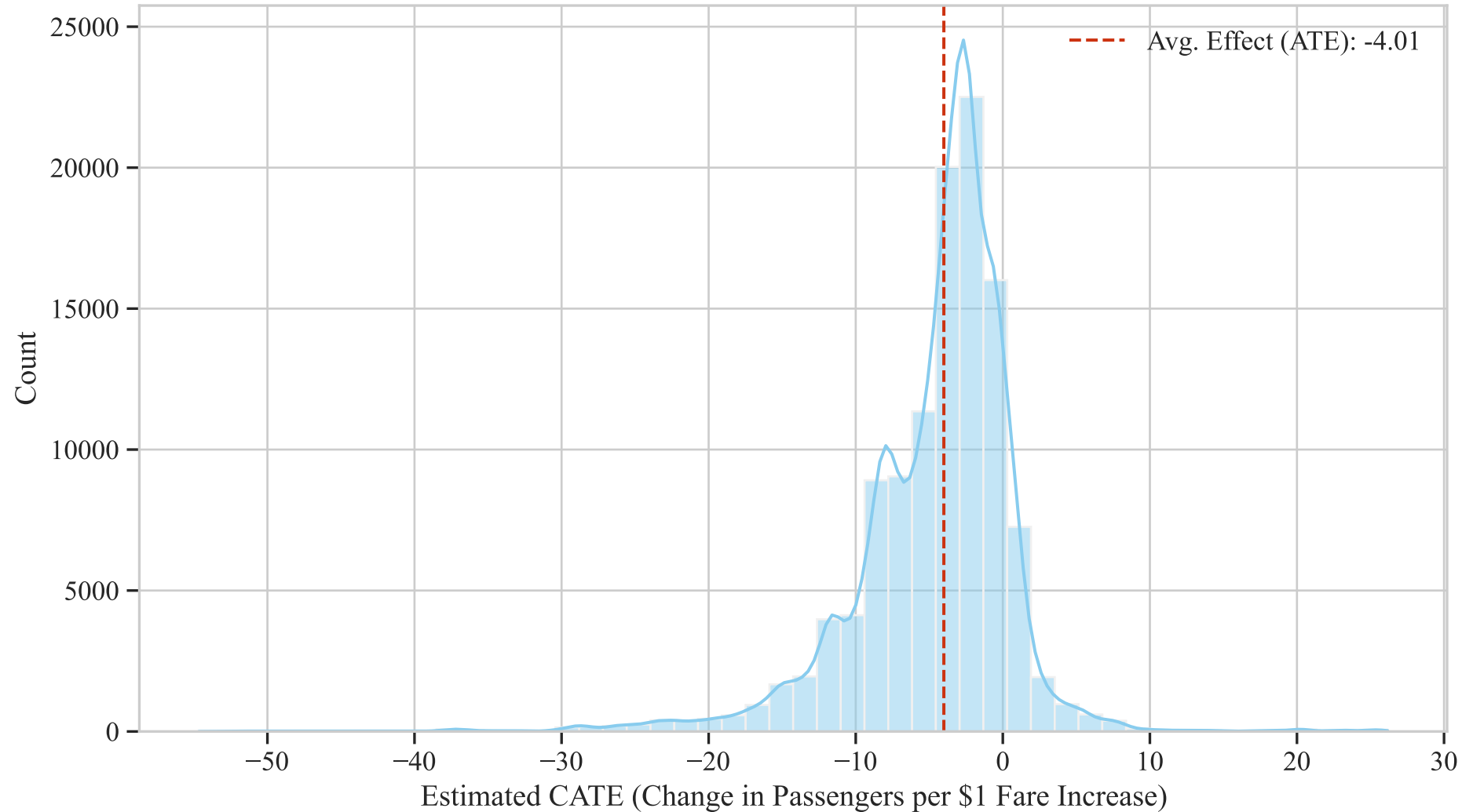
Distribution of Estimated CATEs (Effect of $1 Fare Increase)
