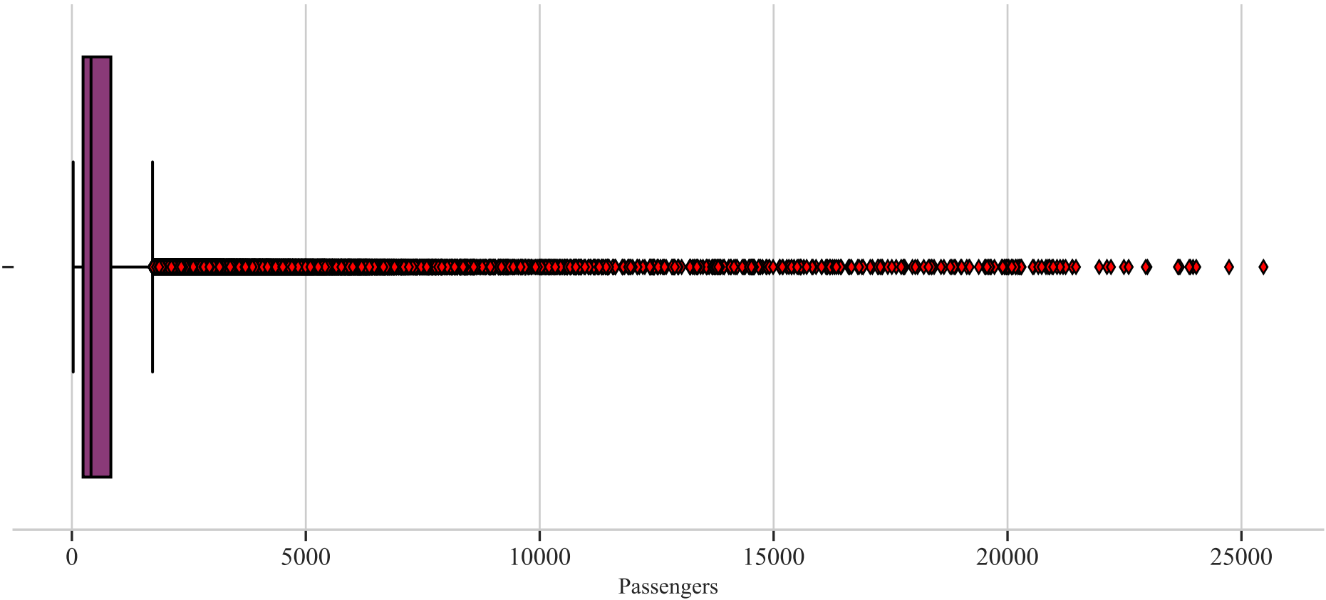
Boxplot for 'Passengers'
