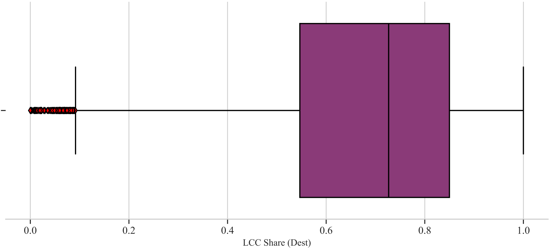
Boxplot for 'LCC Share (Dest)'
