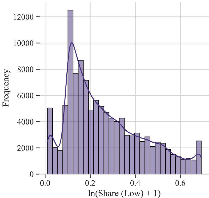
Natural Log-Transformed Distribution of Share (Low)
