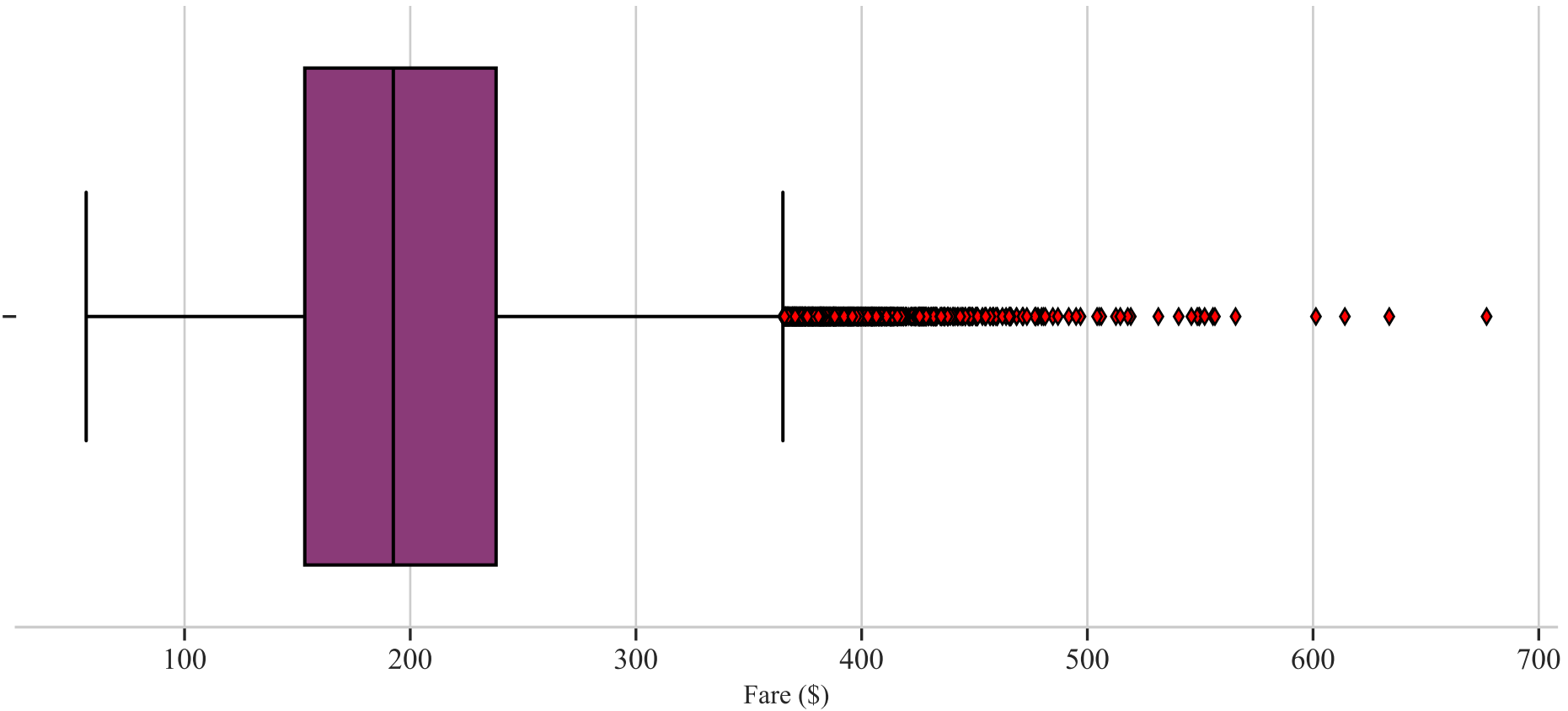
Boxplot for `Fare ($)`
