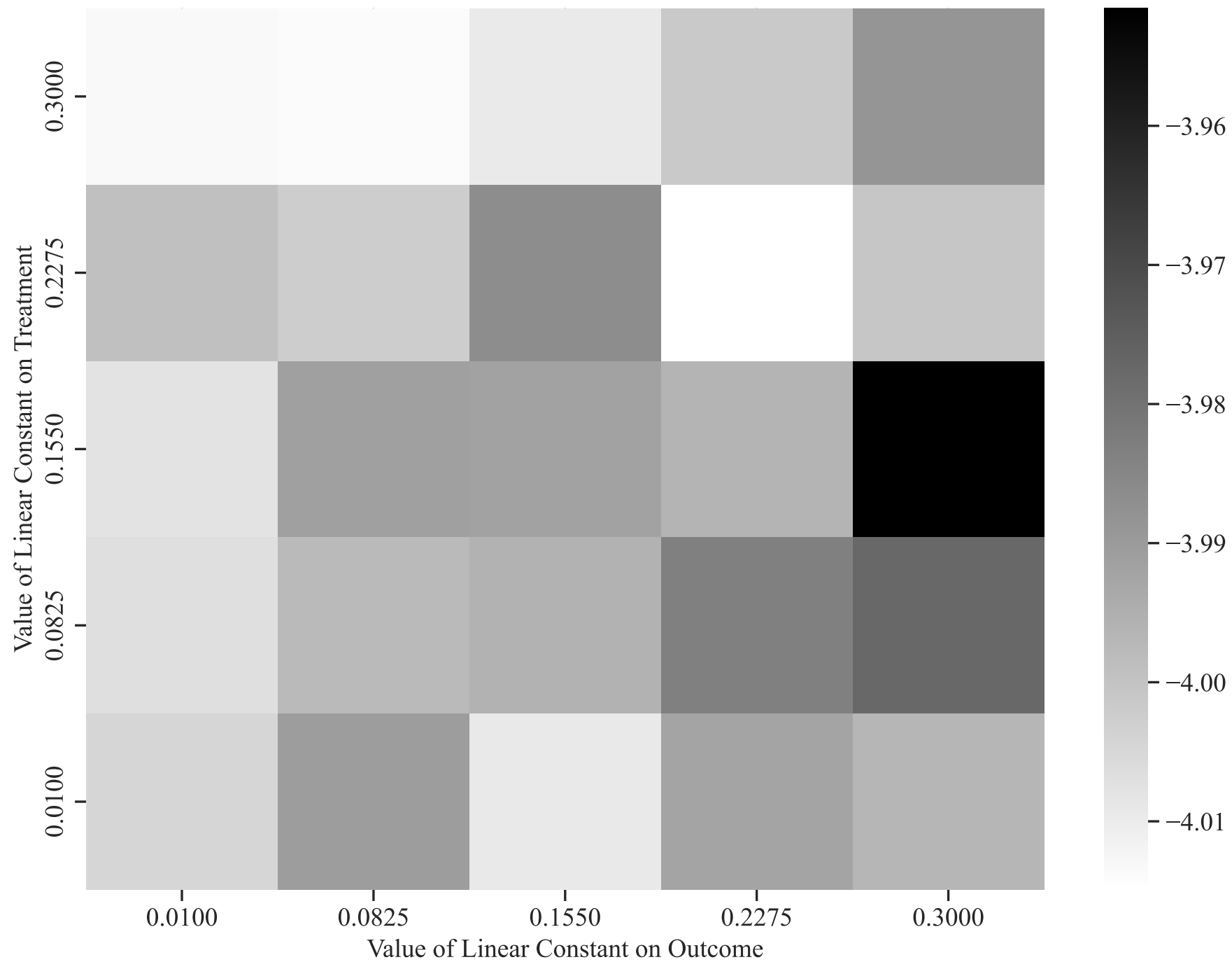
Effect of Unobserved Common Cause on Estimated ATE
