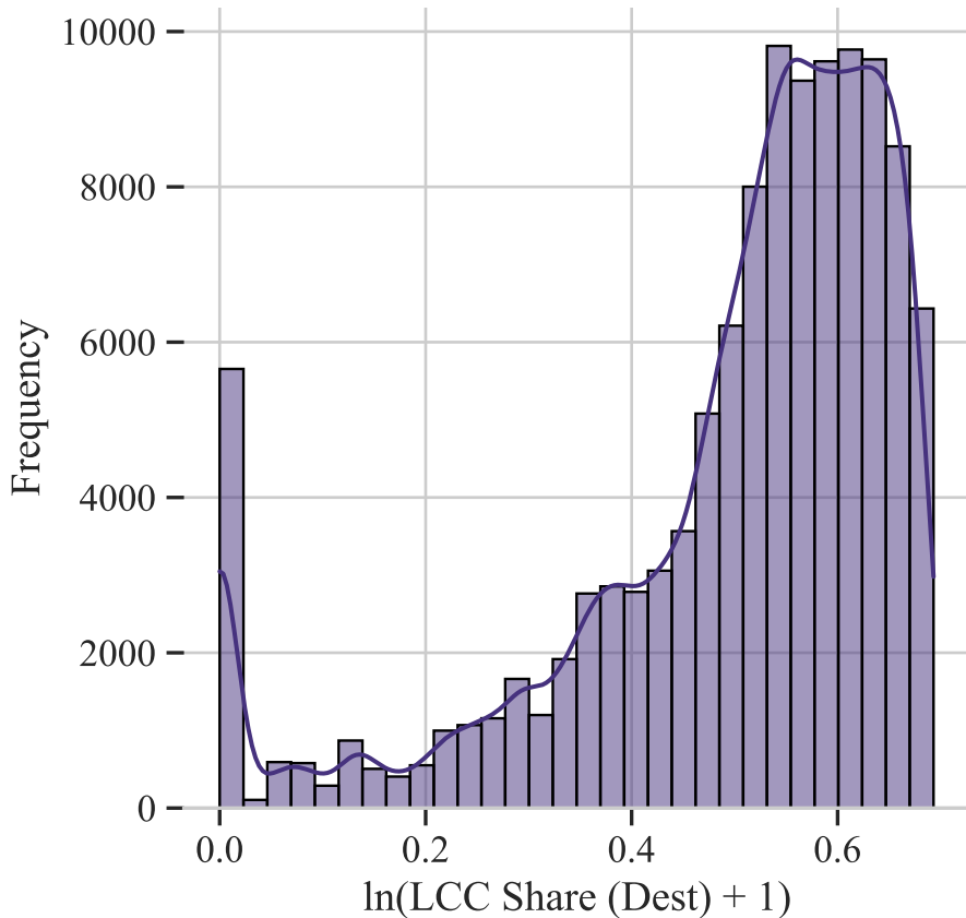
Natural Log-Transformed Distribution of LCC Share (Dest)
