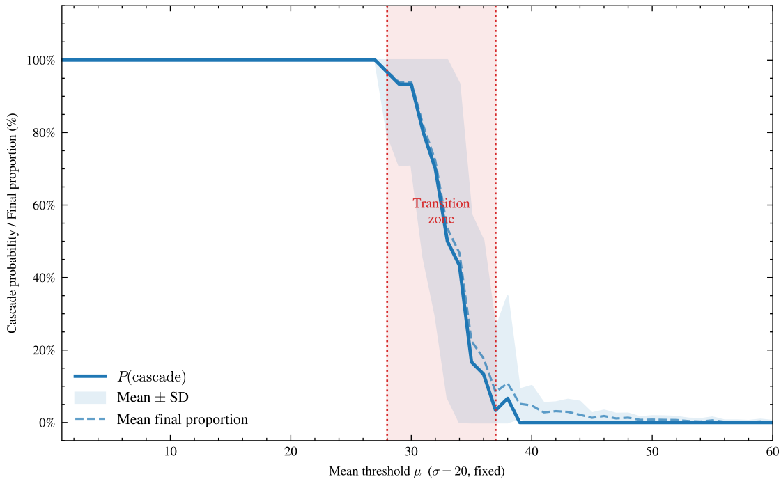
Experiment 1: Effect of Mean Threshold on Collective Action
