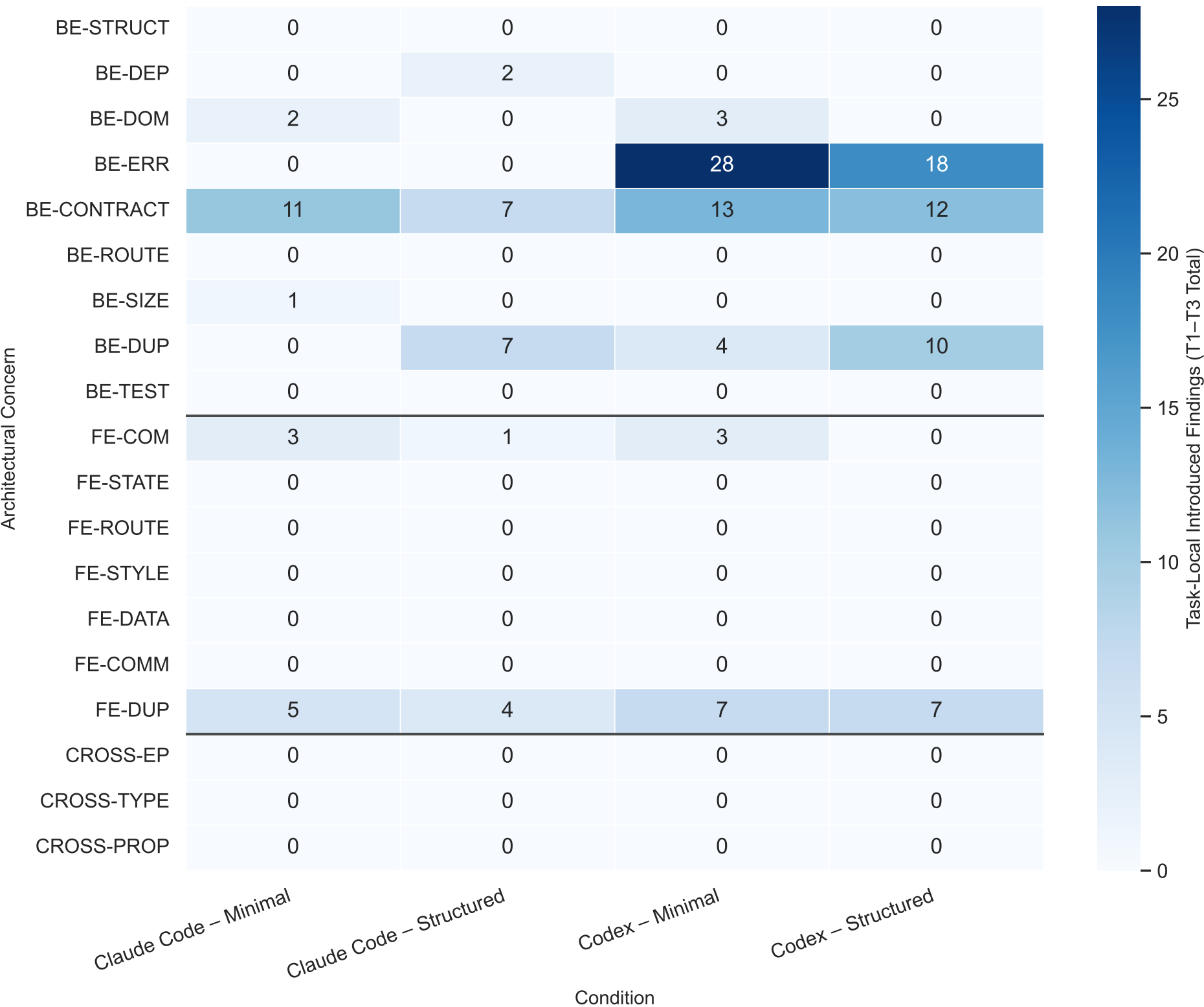
Architectural Concern Profile Task-Local Introduced Findings Summed Across T1–T3
